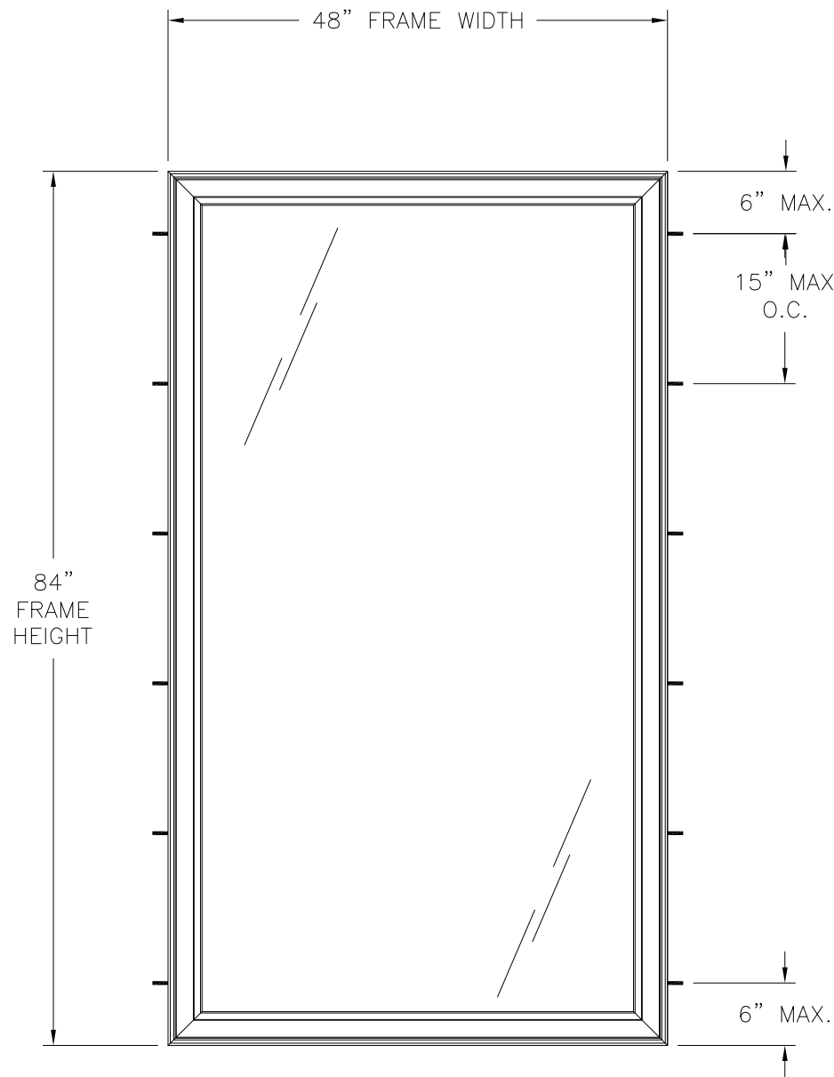
400 VINYL PICTURE WINDOW EXTERIOR VIEW FRAME INSTALLATION
