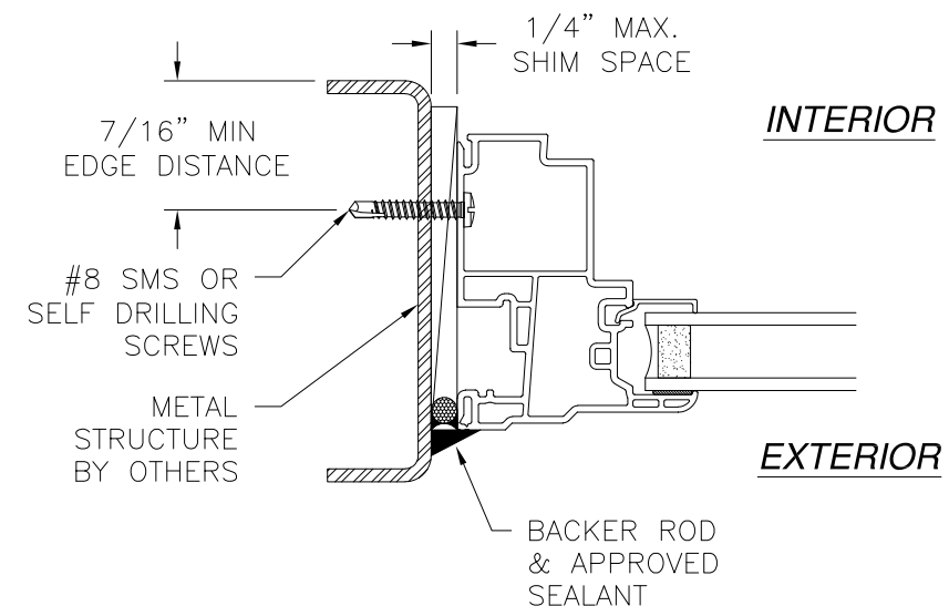
JAMB INSTALLATION DETAIL METAL STRUCTURE INSTALLATION
