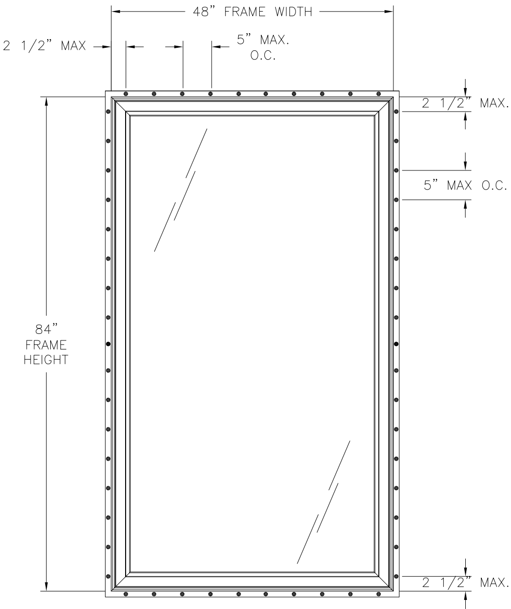
400 VINYL PICTURE WINDOW EXTERIOR VIEW FIN INSTALLATION
