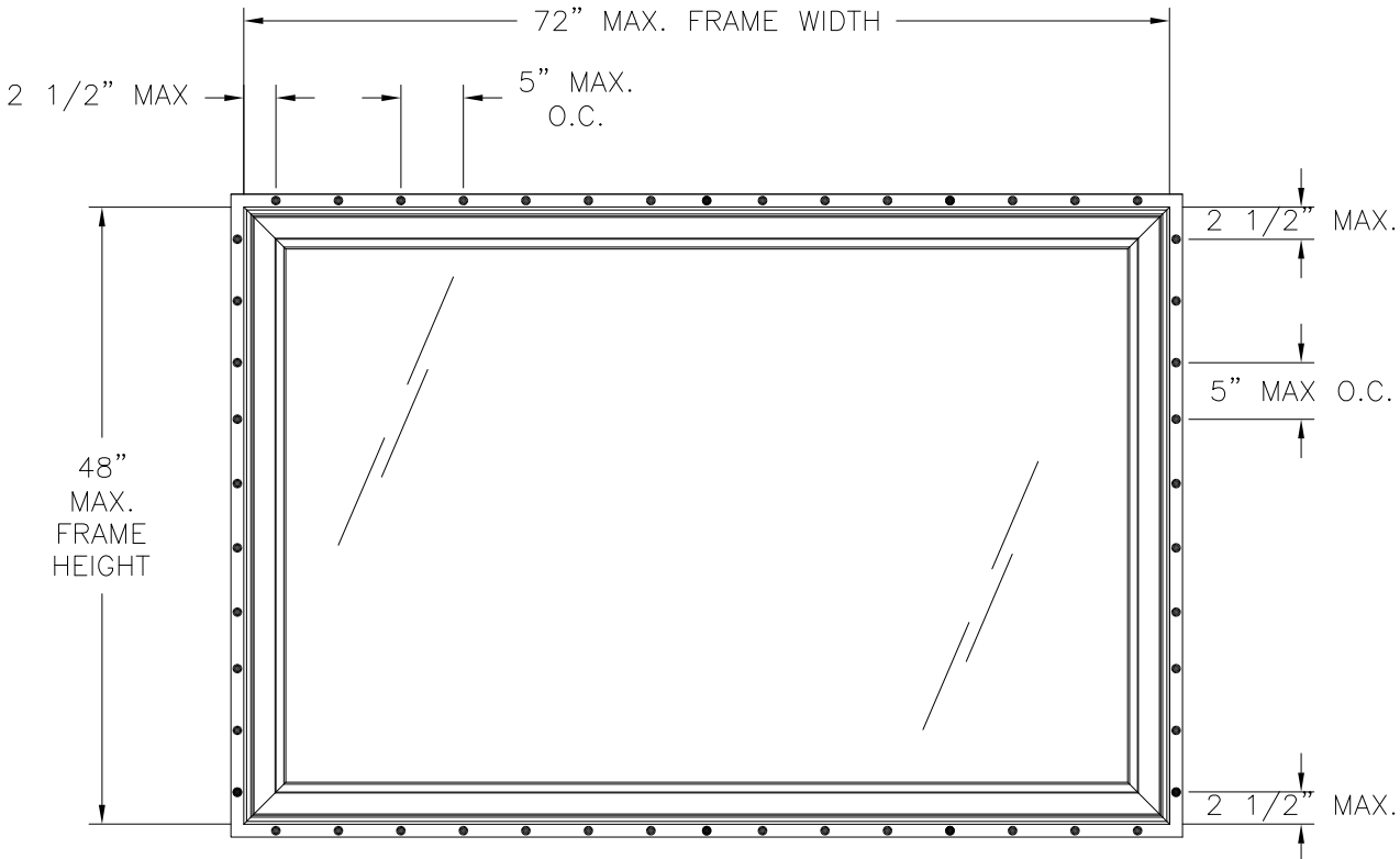
400 VINYL PICTURE WINDOW EXTERIOR VIEW FIN INSTALLATION
