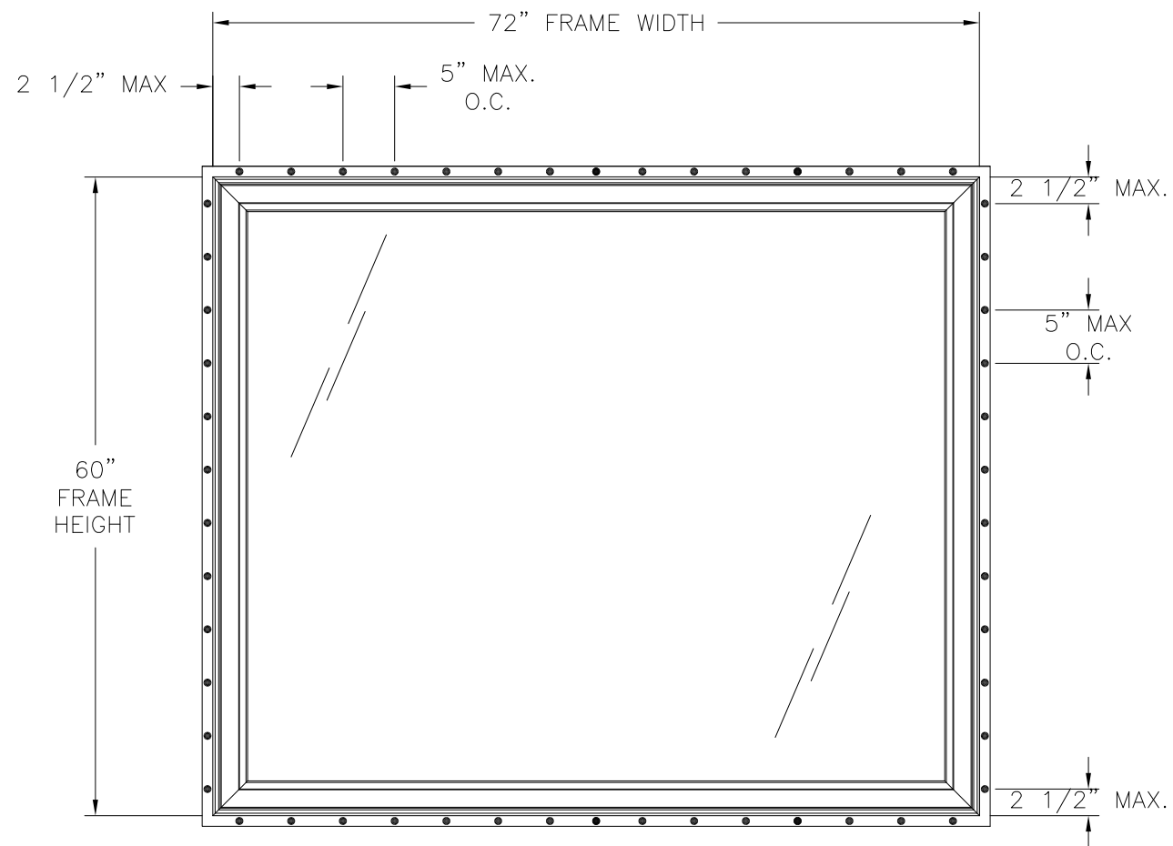
400 VINYL PICTURE WINDOW EXTERIOR VIEW FIN INSTALLATION
