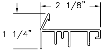
SIDELITE SILL SUPPORT PLASTIC
