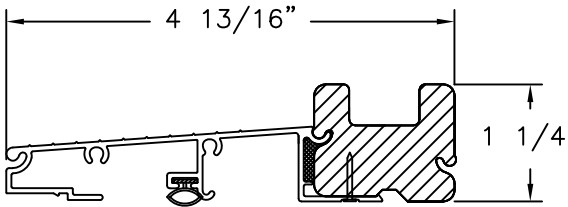
THRESHOLD ALUMINUM / PVC
