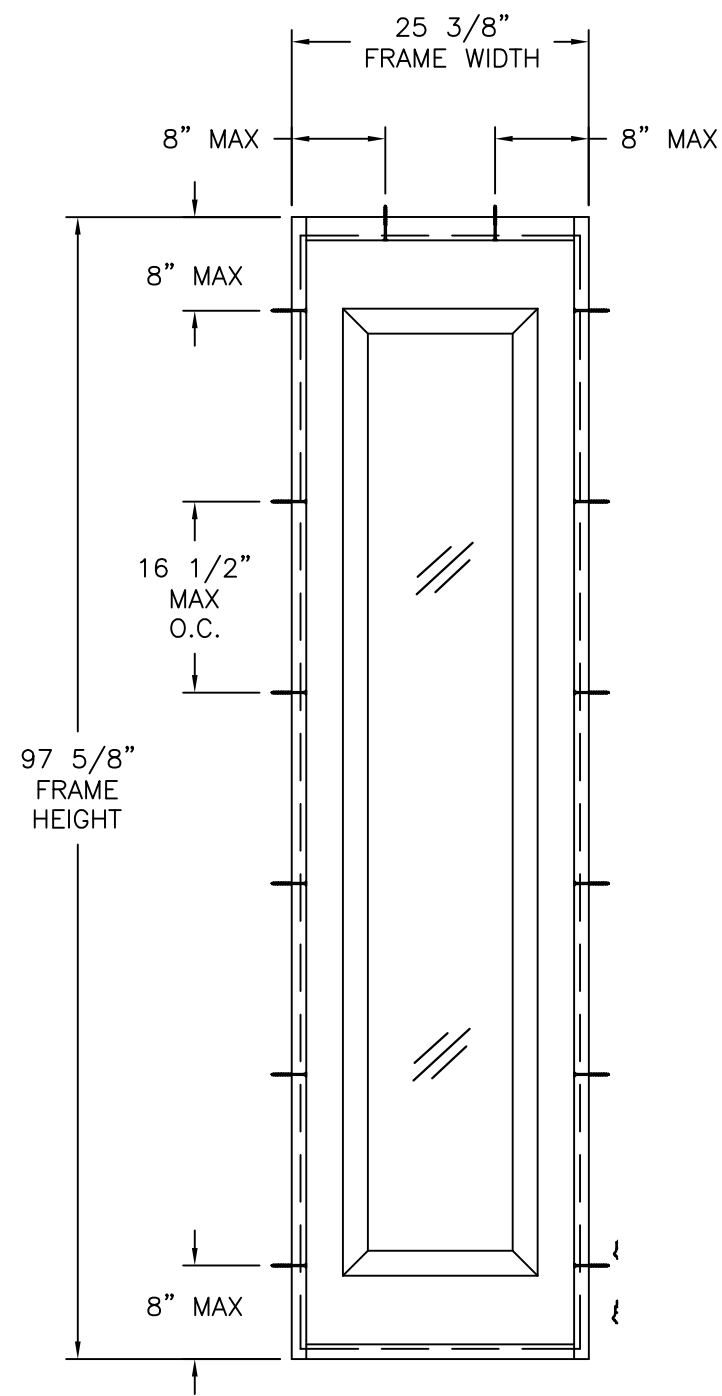
STEEL FIXED SIDELITE WINDOW EXTERIOR VIEW
