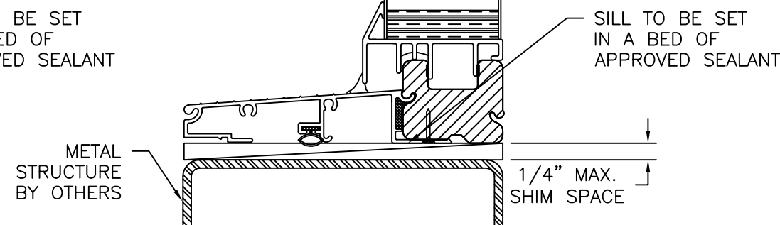
VERTICAL CROSS SECTION METAL STRUCTURE INSTALLATION
