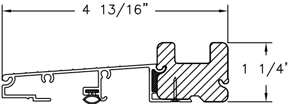
① THRESHOLD ALUMINUM / PVC
