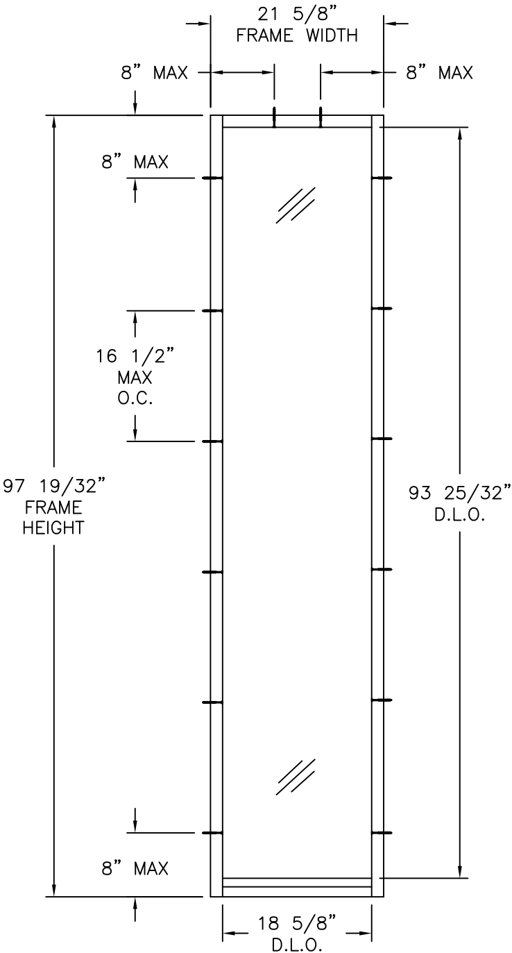
DIRECT SET SIDELITE EXTERIOR VIEW
