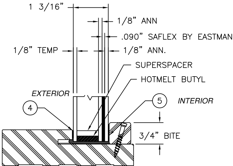
GLAZING DETAIL A
