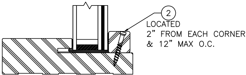
VERTICAL SECTION
