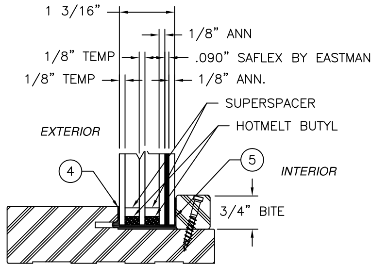
GLAZING DETAIL B
