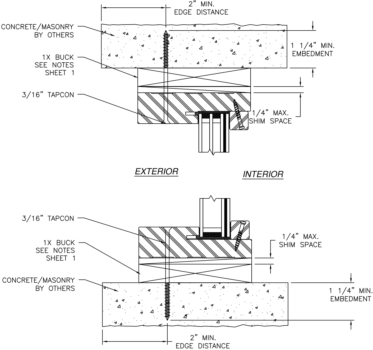
VERTICAL CROSS SECTION CONCRETE/MASONRY INSTALLATION HEAD & SILL SHOWN JAMBS SIMILAR
