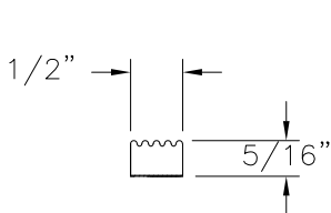
RIBBED GASKET SEAL CLOSED CELL FOAM
