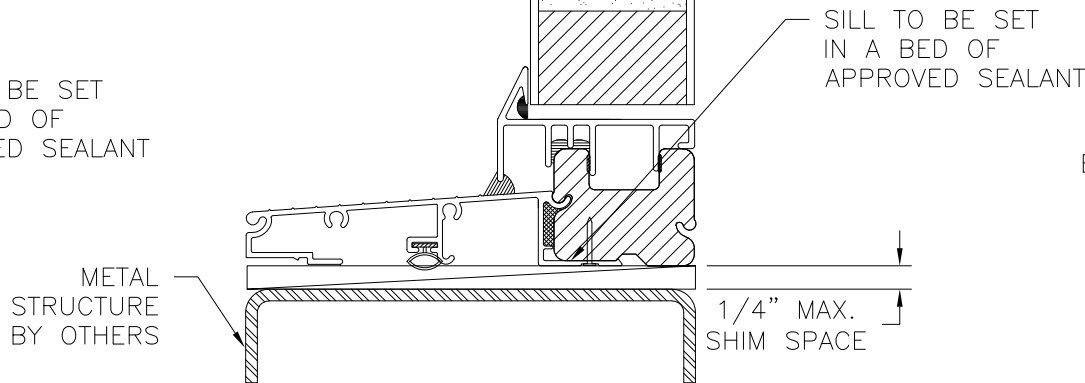
VERTICAL CROSS SECTION METAL STRUCTURE INSTALLATION
