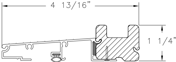
THRESHOLD ALUMINUM / PVC
