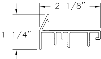
SIDELITE SILL SUPPORT PLASTIC
