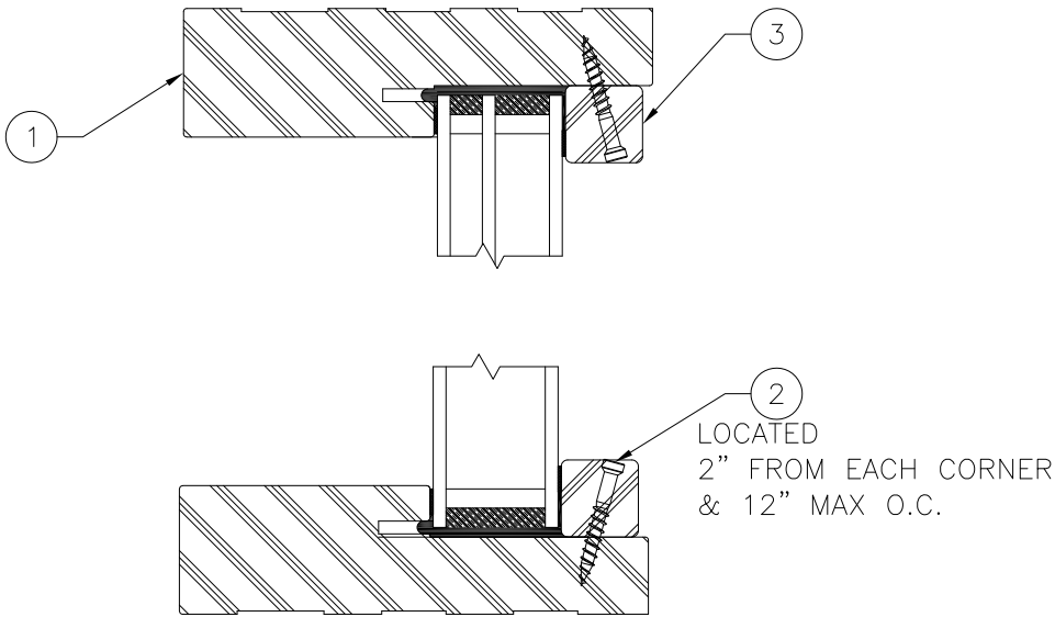
VERTICAL SECTION
