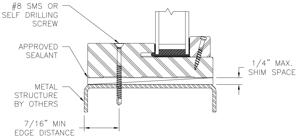
VERTICAL CROSS SECTION METAL STRUCTURE INSTALLATION HEAD & SILL SHOWN JAMBS SIMILAR
