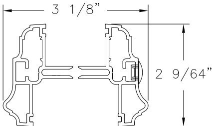
3 GLASS TRIM ALUMINUM
