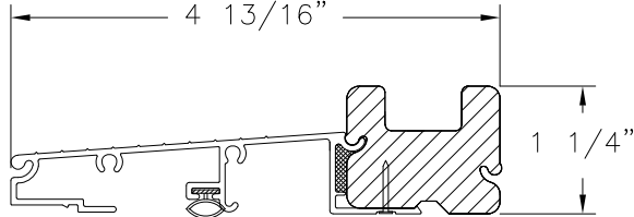
1 THRESHOLD ALUMINUM / PVC
