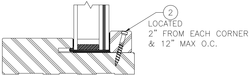
VERTICAL SECTION
