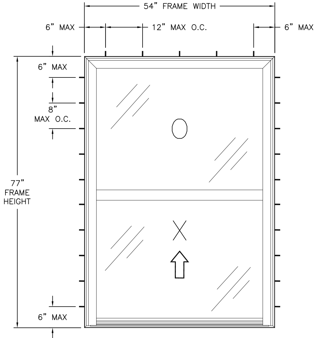
SERIES 176 SH VINYL SINGLE HUNG WINDOW EXTERIOR VIEW THROUGH FRAME INSTALLATION FOR WOOD FRAMING
