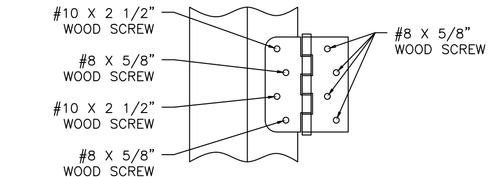
HINGE INSTALLATION DETAIL 2X BUCK/WOOD FRAMING
