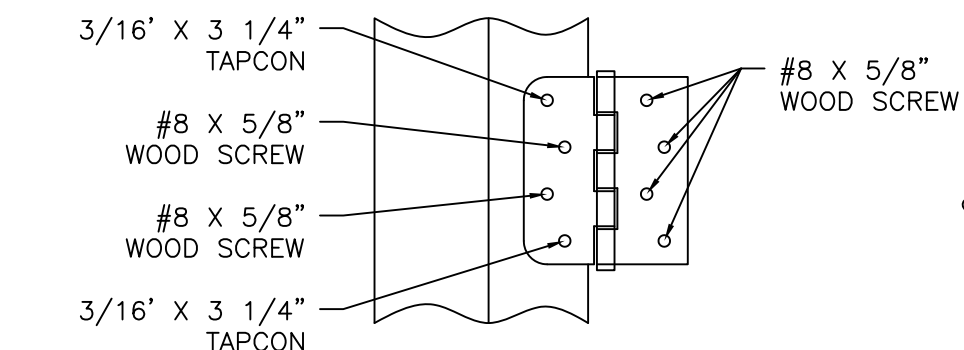
HINGE INSTALLATION DETAIL MASONRY/CONCRETE
