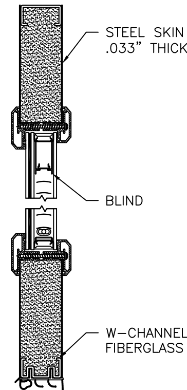
PANEL OPTION 25 SEVERE WEATHER DUAL GLAZED BLINDS
