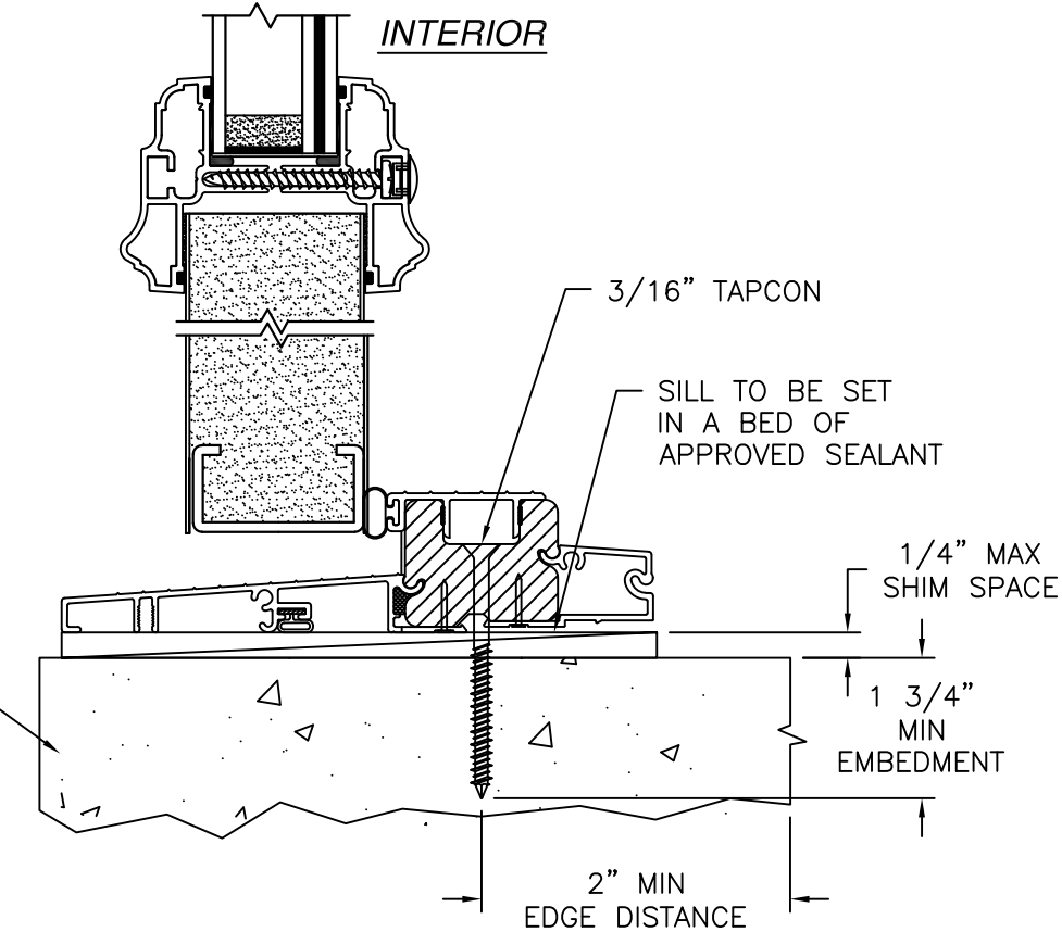
VERTICAL CROSS SECTION CONCRETE/MASONRY INSTALLATION
