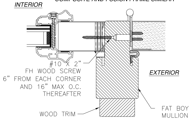
DETAIL A WITH FAT BOY MULLION
