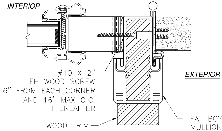
DETAIL A WITH HYBRID FAT BOY MULLION
