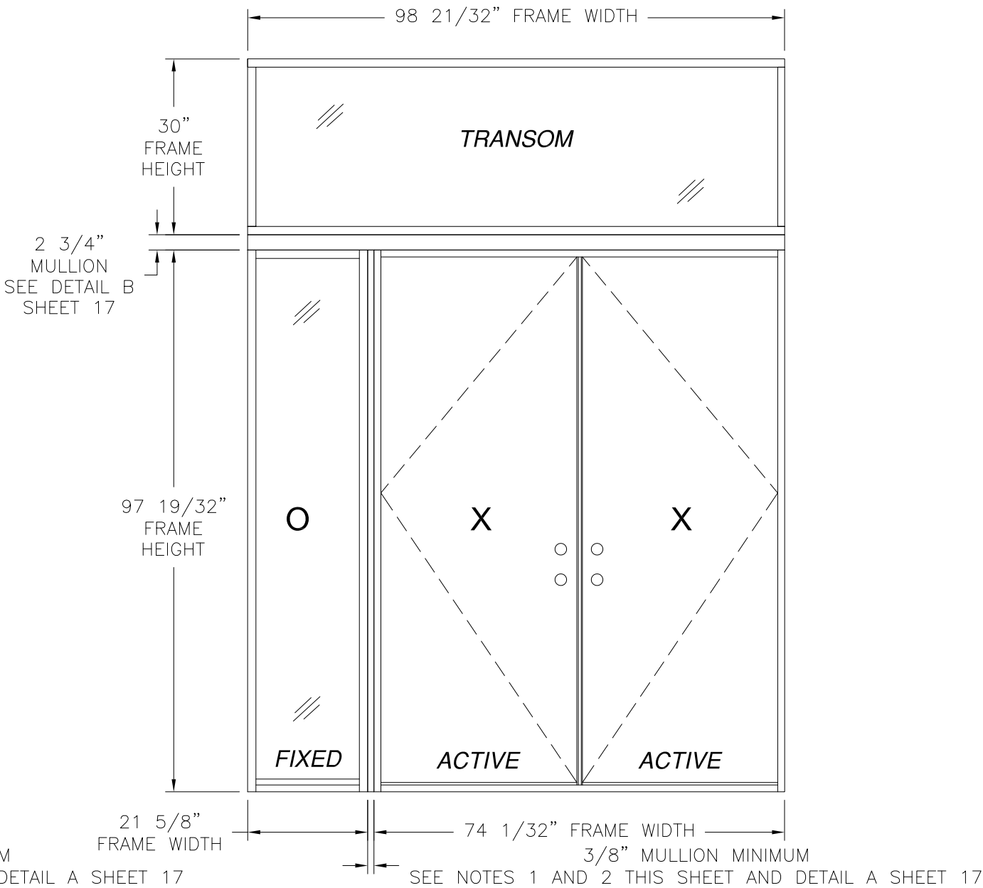
DOUBLE DOOR W/ DIRECT SET SIDELITE AND TRANSOM EXTERIOR VIEW OXX SHOWN XXO ALSO APPROVED
