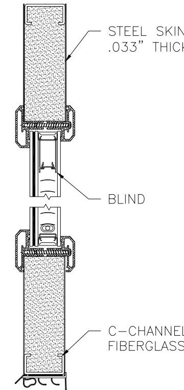
PANEL OPTION 26 SEVERE WEATHER DUAL GLAZED BLINDS
