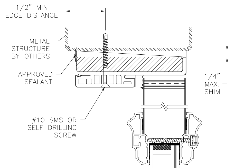
VERTICAL CROSS SECTION SIDELITE INSTALLATION METAL STRUCTURE STANDARD SIDELITE SHOWN DIRECT SET SIDELITE SIMILAR
