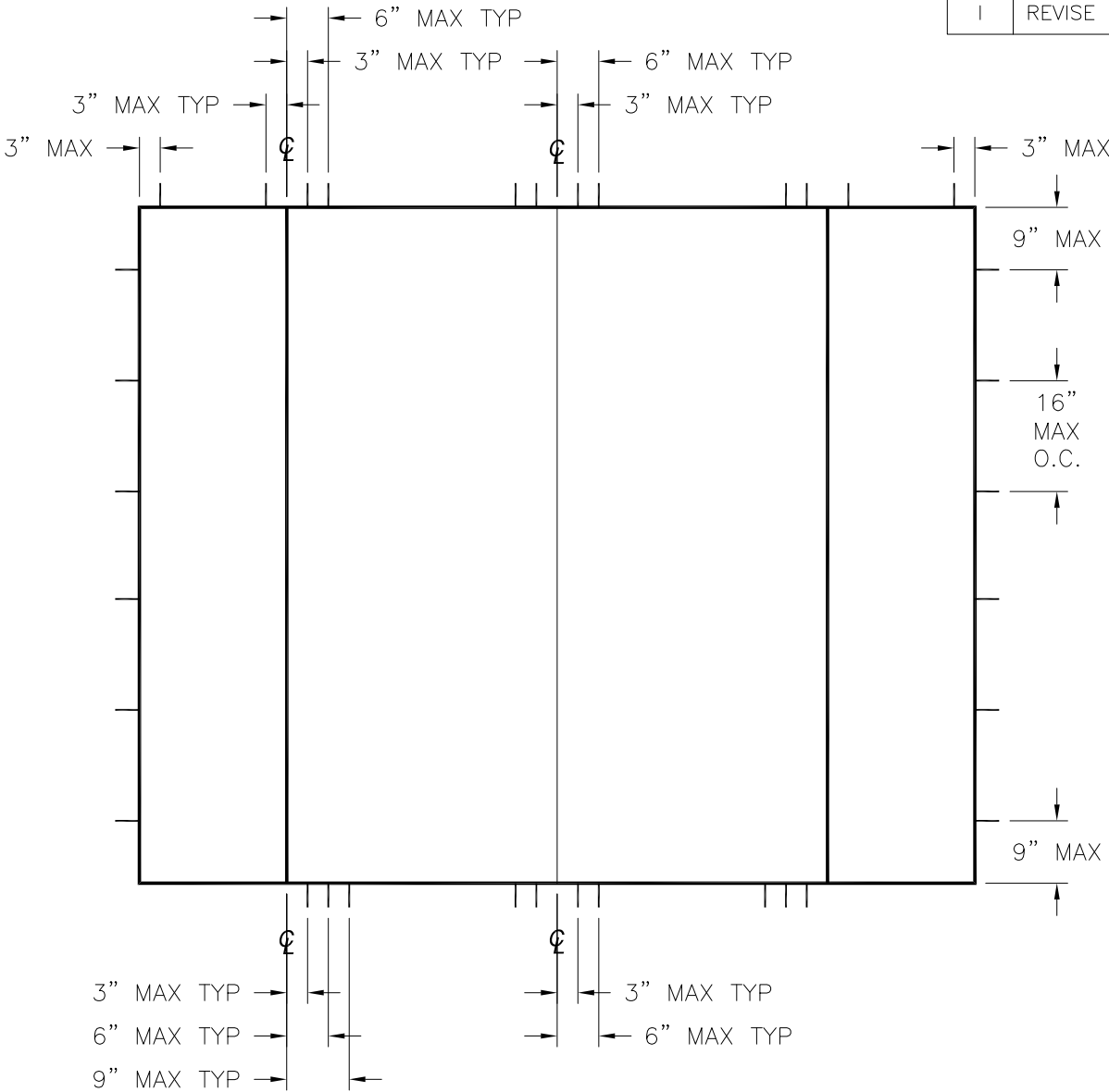
DOUBLE DOOR WITH SIDELITES
