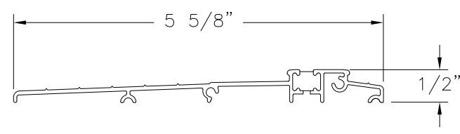
ADA THRESHOLD
