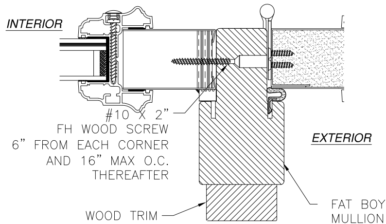
DETAIL C WITH FAT BOY MULLION
