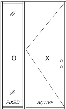
SINGLE DOOR W/ DIRECT SET SIDELITE EXTERIOR VIEW
