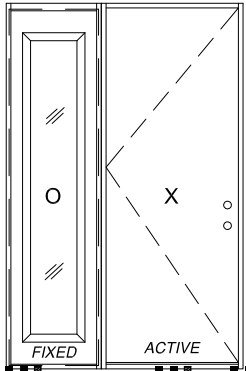
SINGLE DOOR W/ STD SIDELITE EXTERIOR VIEW
