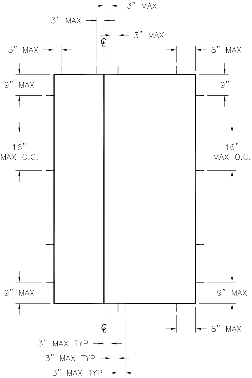
SINGLE W/SIDELITE
