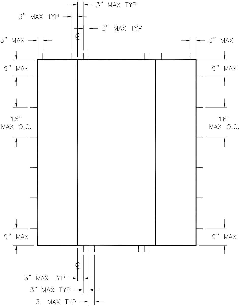
SINGLE W/SIDELITES
