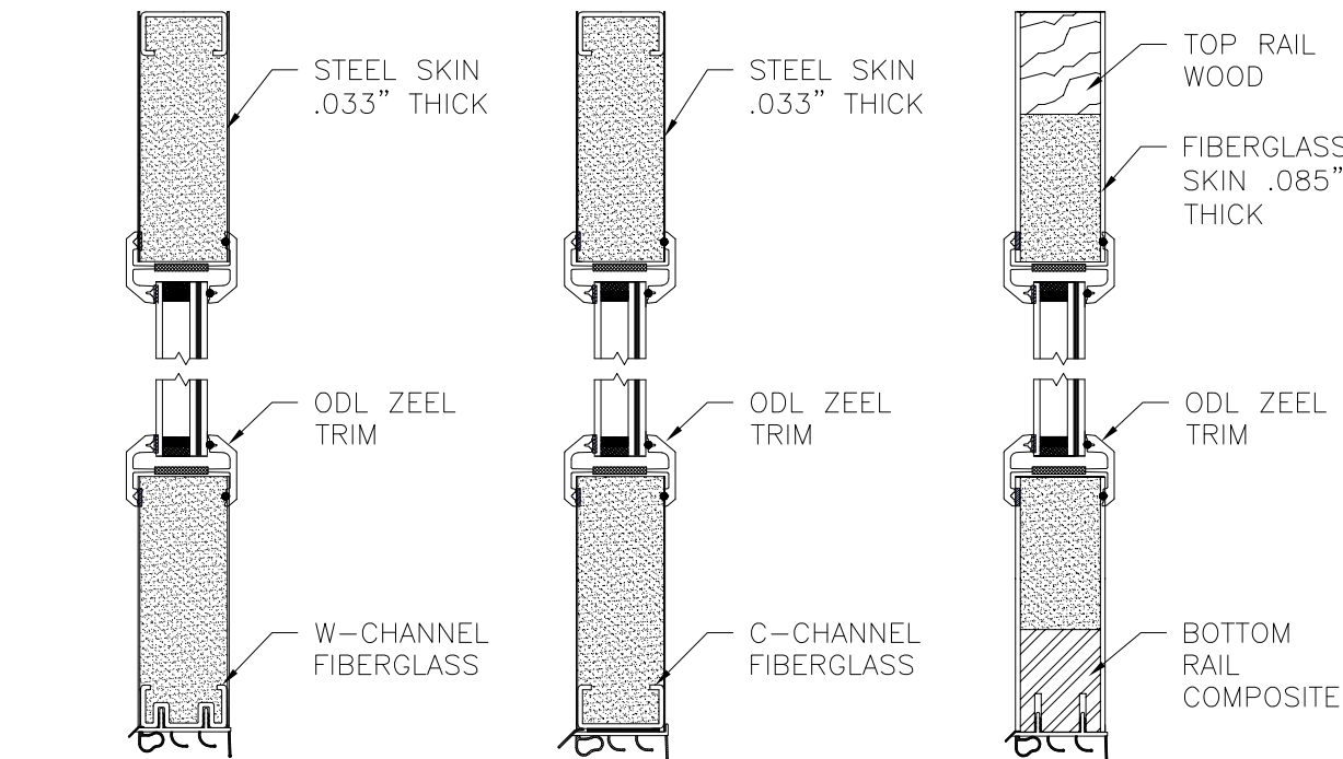
PANEL OPTION 19
