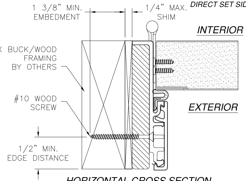
HORIZONTAL CROSS SECTION DOOR INSTALLATION - 2X BUCK/WOOD FRAMING
