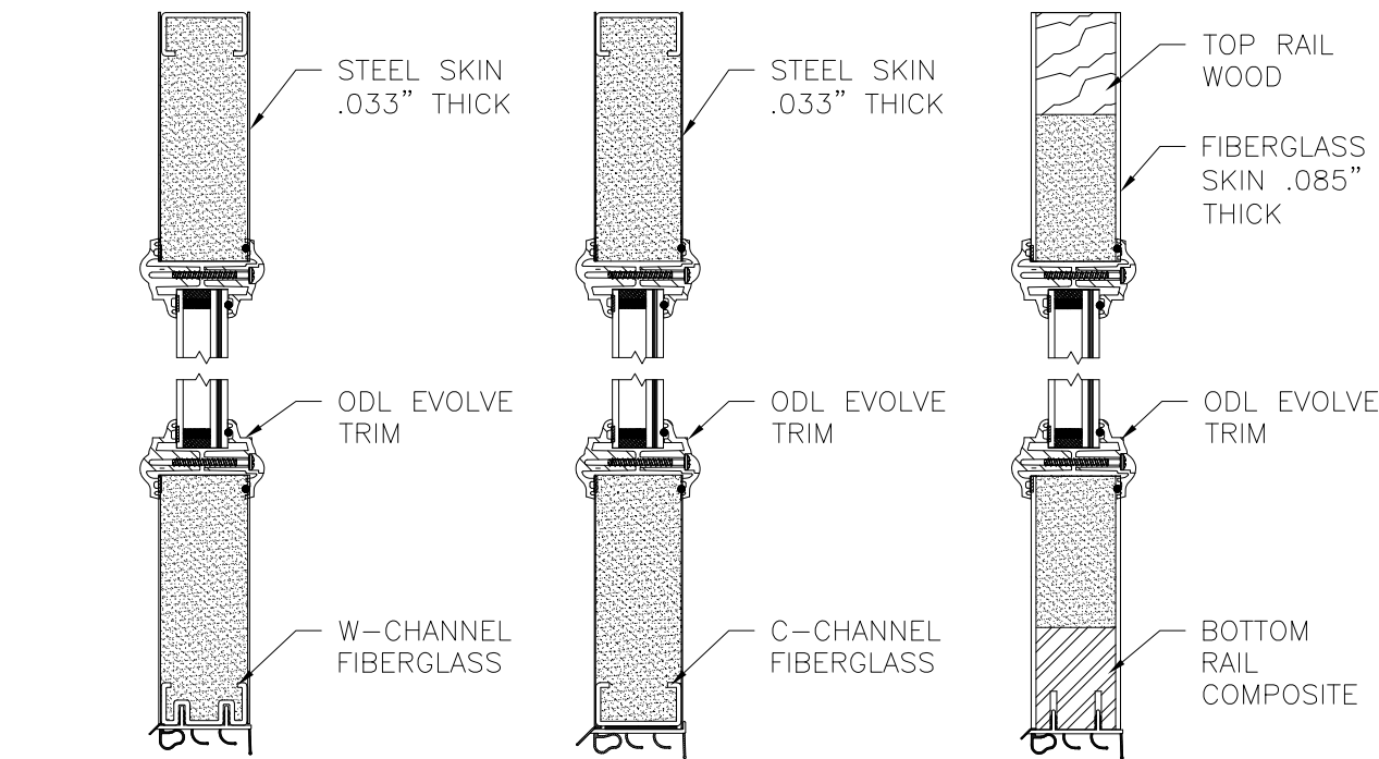
PANEL OPTION 22
