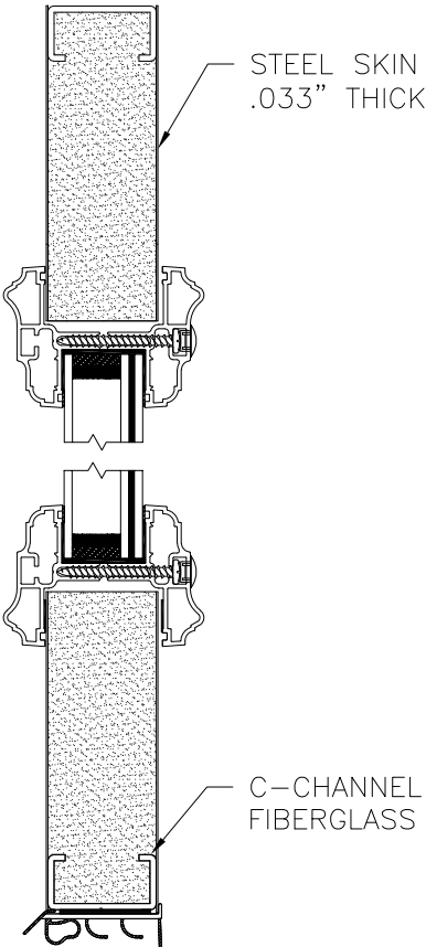
PANEL OPTION 2
