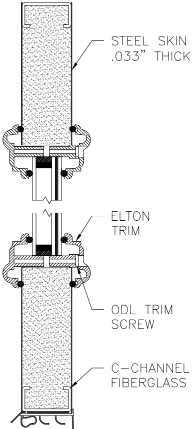
PANEL OPTION 10
