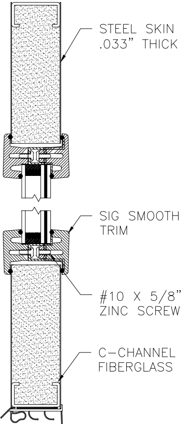
PANEL OPTION 4
