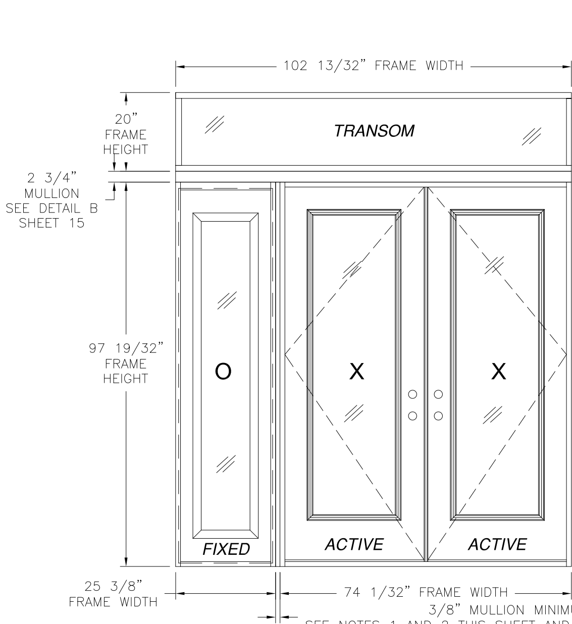
DOUBLE DOOR W/ STD SIDELITE AND TRANSOM EXTERIOR VIEW OXX SHOWN XXO ALSO APPROVED
