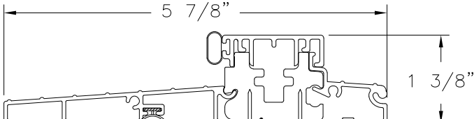
STANDARD OUTSWING THRESHOLD
