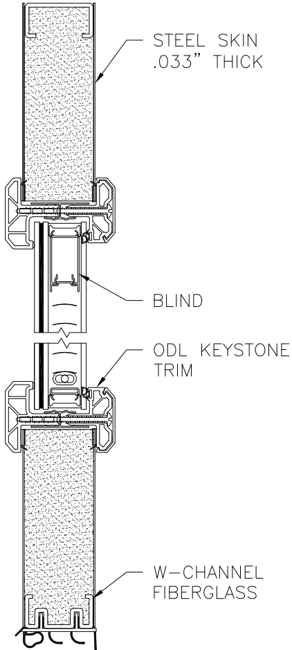
PANEL OPTION 15
