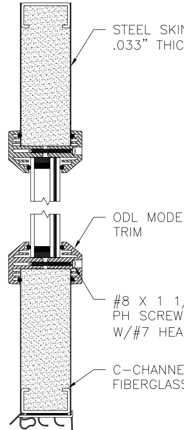
PANEL OPTION 8
