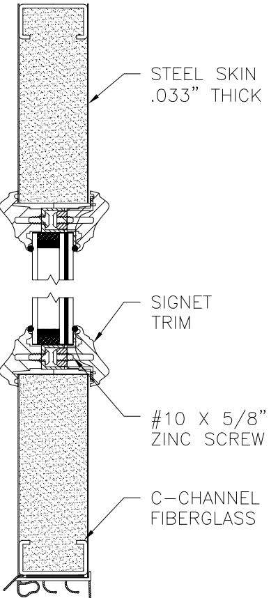
PANEL OPTION 6
