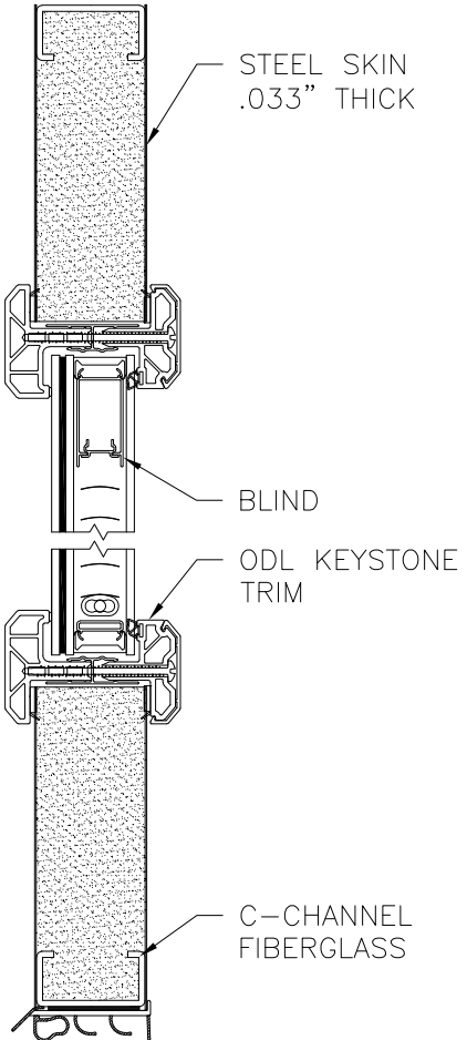
PANEL OPTION 16
