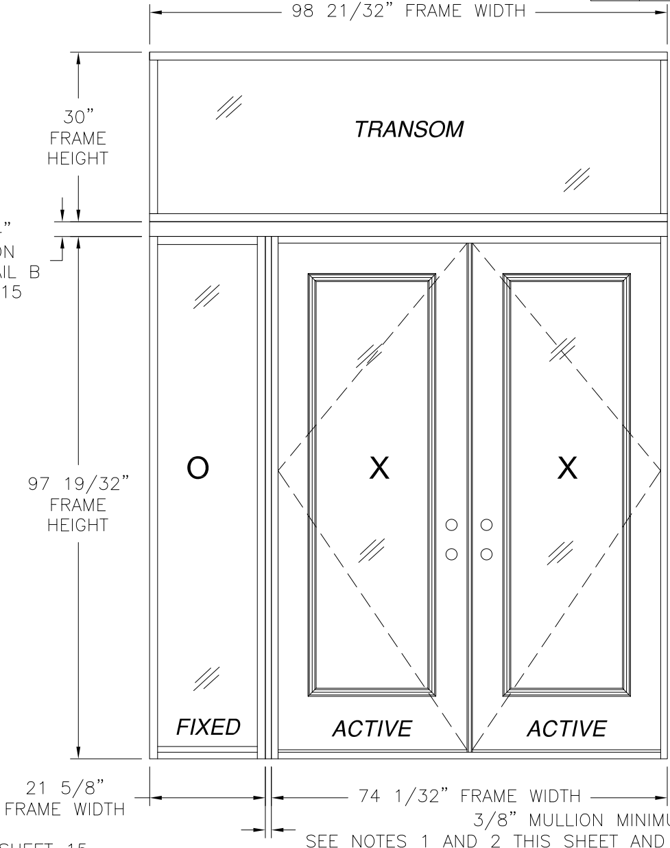
DOUBLE DOOR W/ DIRECT SET SIDELITE AND TRANSOM EXTERIOR VIEW OXX SHOWN XXO ALSO APPROVED
