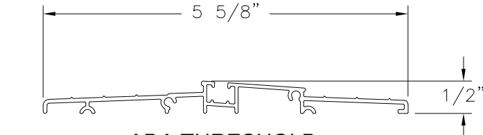
ADA THRESHOLD
