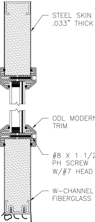
PANEL OPTION 7
