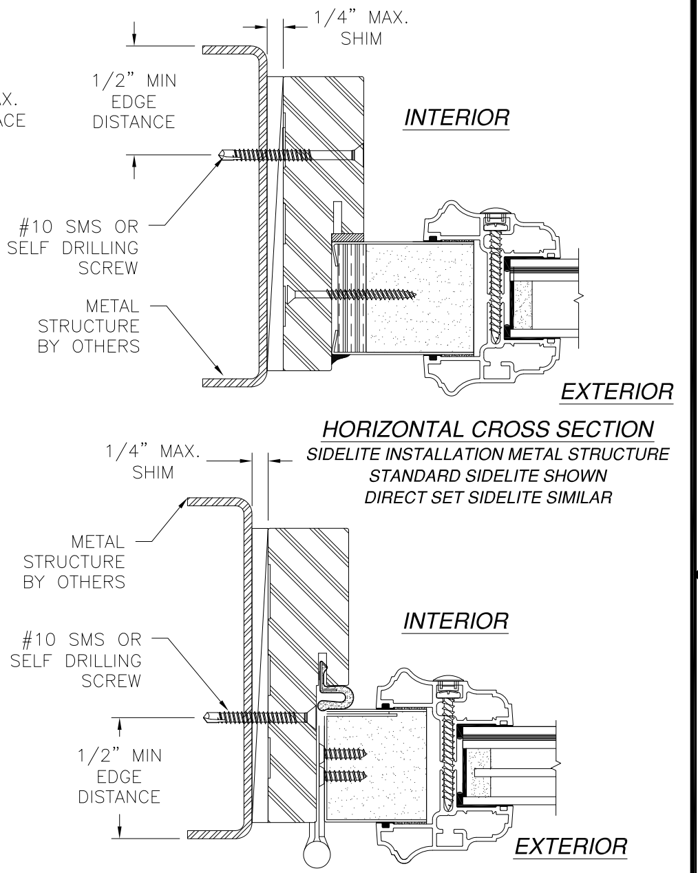
HORIZONTAL CROSS SECTION DOOR INSTALLATION METAL STRUCTURE SIGNED: 08/27/2024
