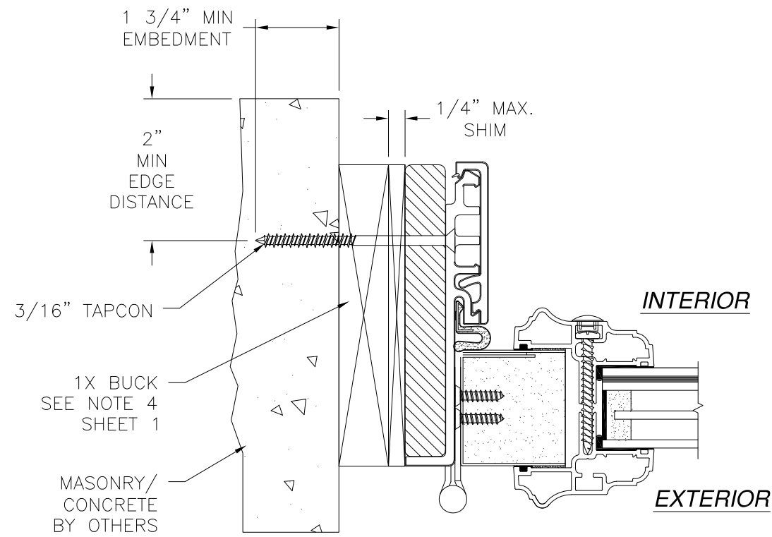
JAMB INSTALLATION DETAIL DOOR INSTALLATION - CONCRETE/MASONRY
