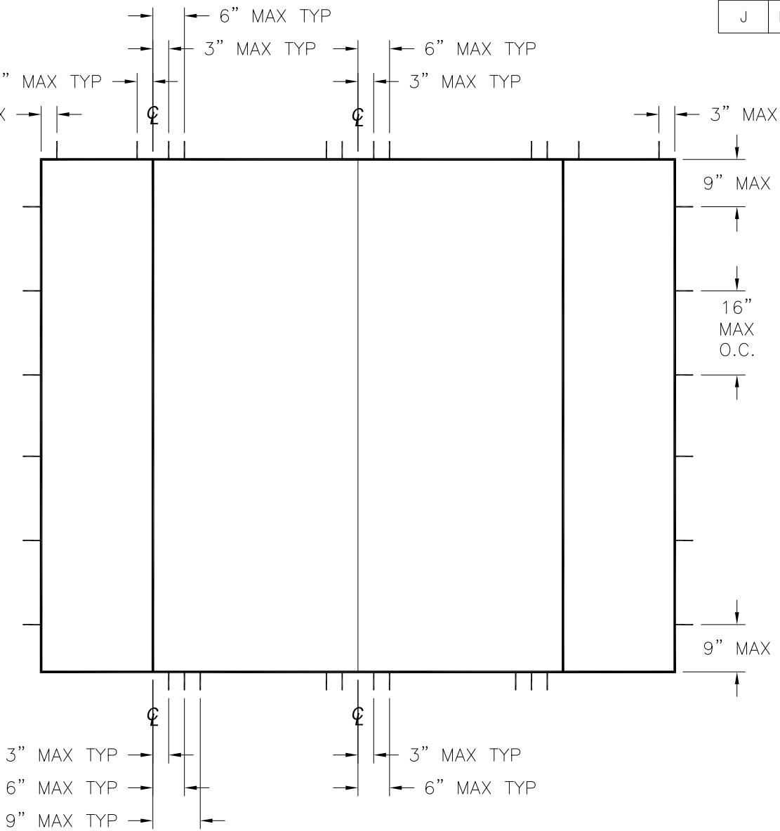
DOUBLE DOOR WITH SIDELITES
