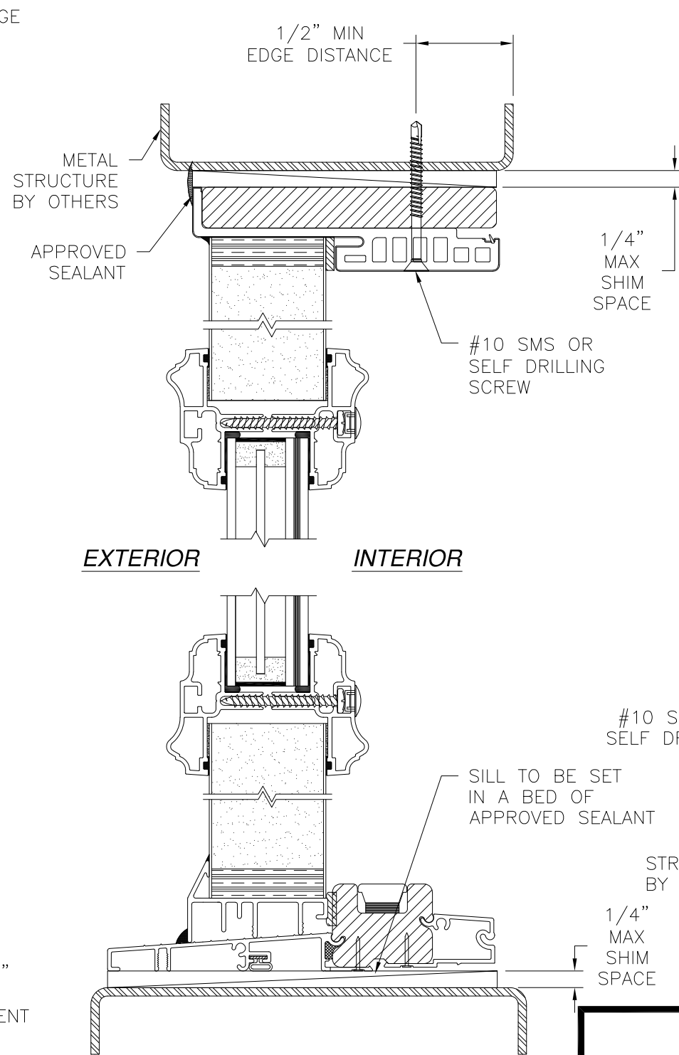
VERTICAL CROSS SECTION SIDELITE INSTALLATION METAL STRUCTURE STANDARD SIDELITE SHOWN DIRECT SET SIDELITE SIMILAR
