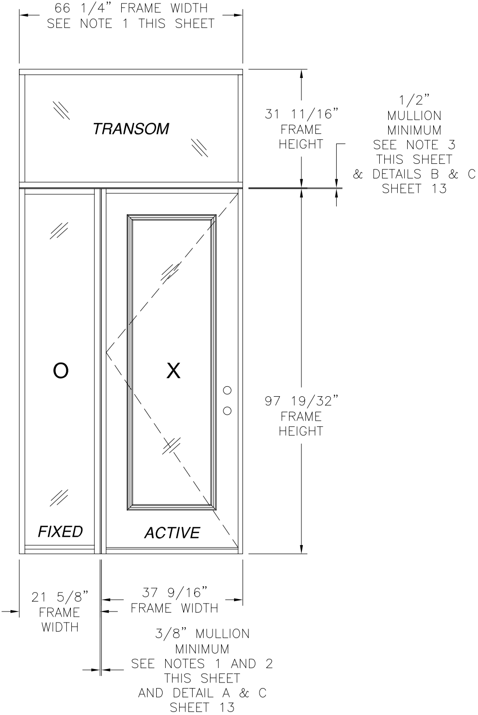
SINGLE DOOR W/ DIRECT SET SIDELITE AND TRANSOM EXTERIOR VIEW OX SHOWN XO ALSO APPROVED
