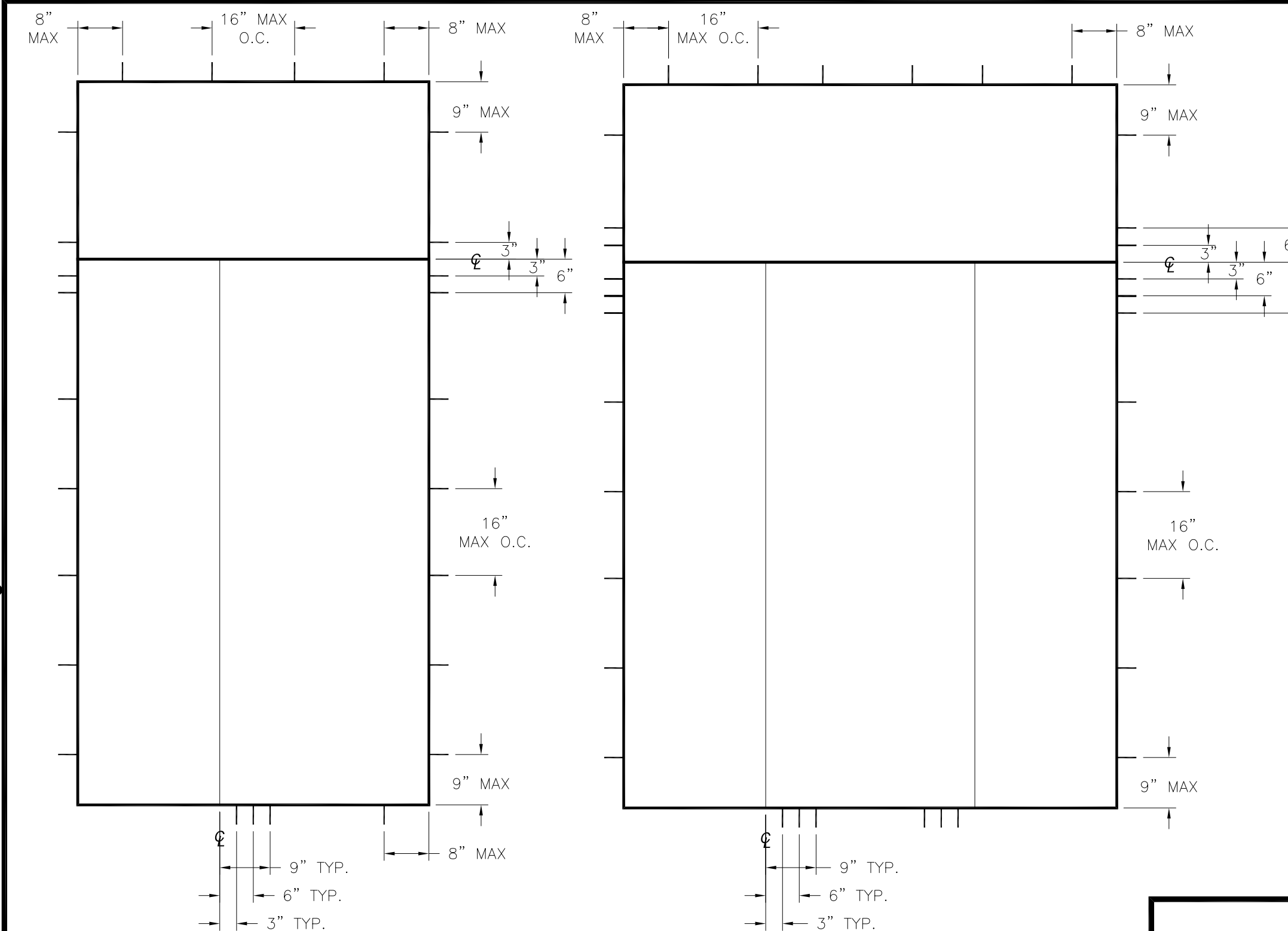
SINGLE W/SIDELITE AND TRANSOM
