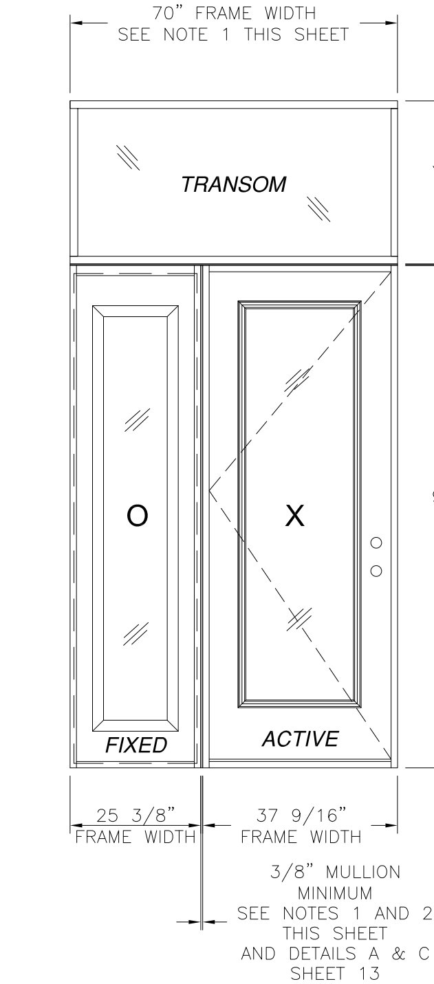
SINGLE DOOR W/ STD SIDELITE AND TRANSOM EXTERIOR VIEW OX SHOWN XO ALSO APPROVED
