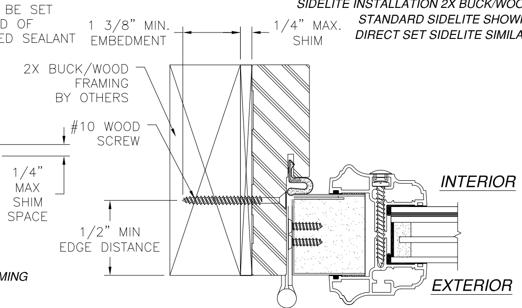
HORIZONTAL CROSS SECTION DOOR INSTALLATION - 2X BUCK/WOOD FRAMING SIGNED: 08/27/2024
