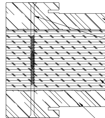
DETAIL B HORIZONTAL MULLION STANDARD FRAME SHOWN, COMPOSITE AND FUSION FRAME SIMILAR
