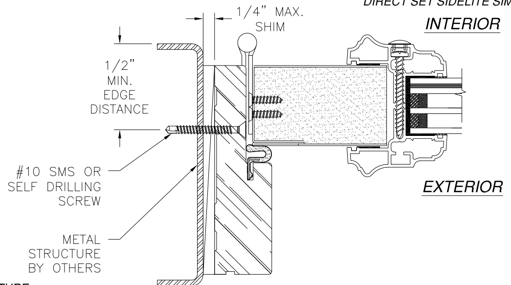
HORIZONTAL CROSS SECTION DOOR INSTALLATION METAL STRUCTURE SIGNED: 08/27/2024
