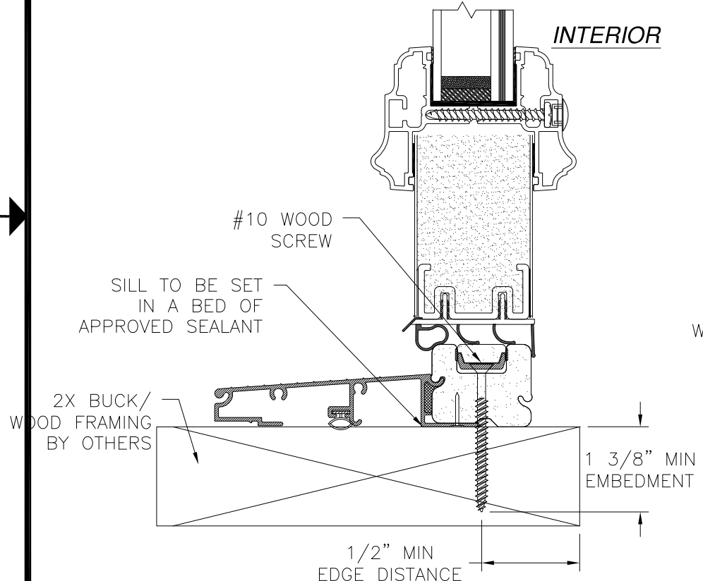
VERTICAL CROSS SECTION DOOR AND TRANSOM INSTALLATION - 2X BUCK/WOOD FRAMING
