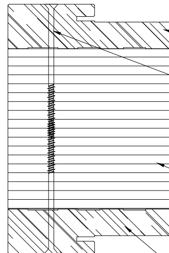
DETAIL C HORIZONTAL MULLION STANDARD FRAME SHOWN, COMPOSITE AND FUSION FRAME SIMILAR
