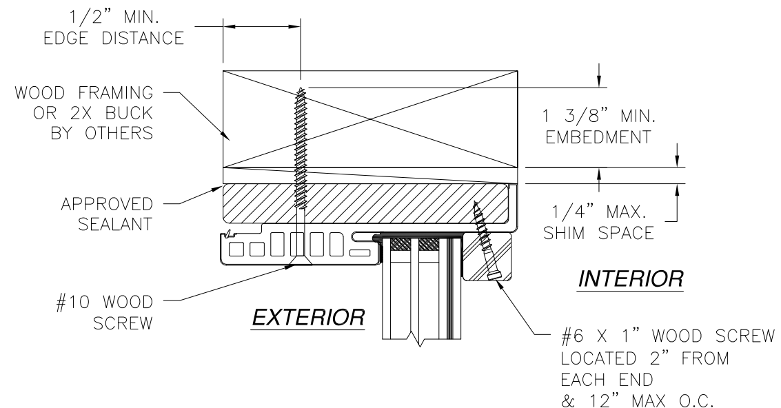
VERTICAL CROSS SECTION TRANSOM INSTALLATION 2X BUCK/WOOD FRAMING TRANSOM HEAD SHOWN TRANSOM JAMB SIMILAR
