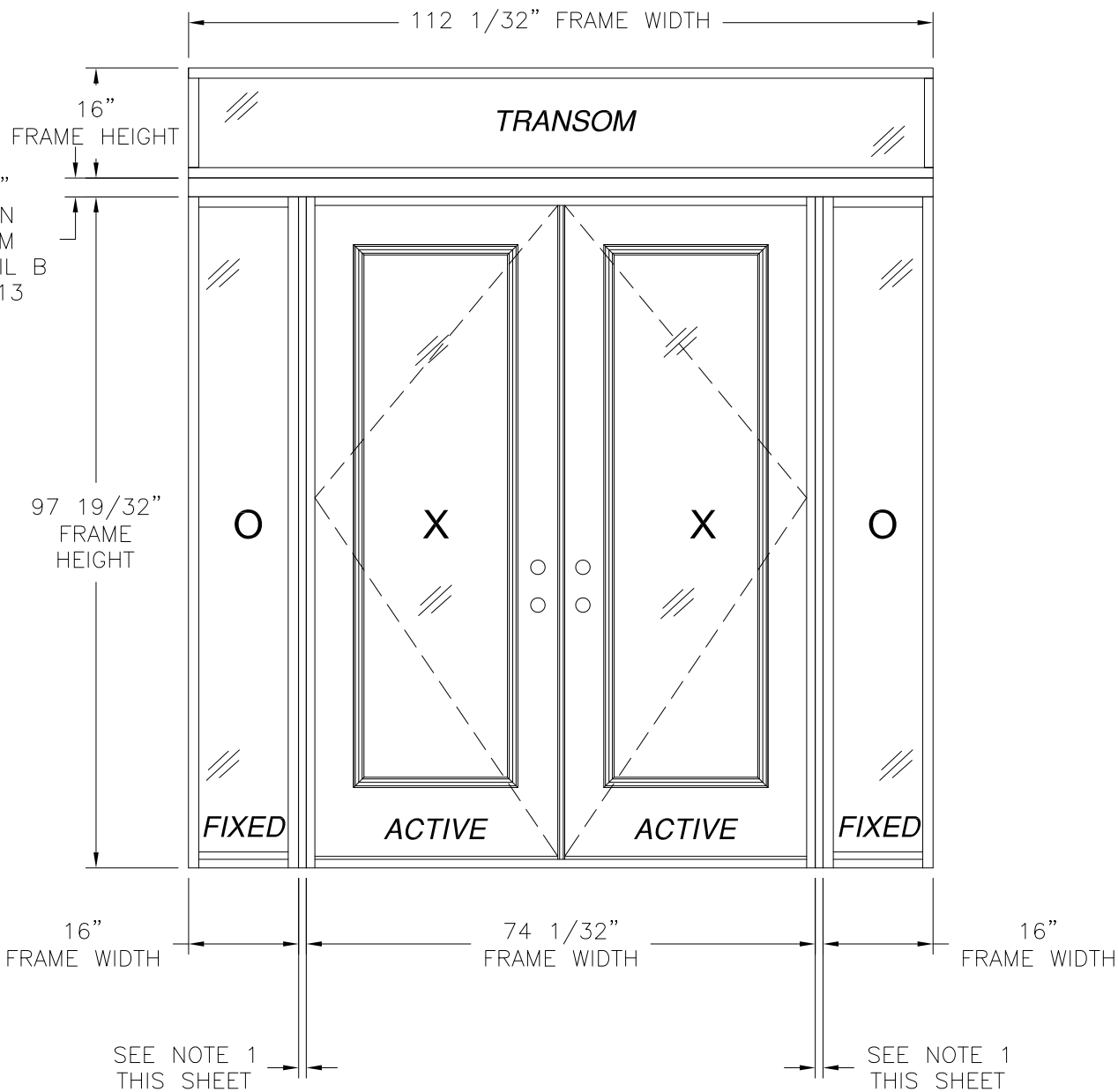
DOUBLE DOOR W/ DIRECT SET SIDELITES AND TRANSOM EXTERIOR VIEW
