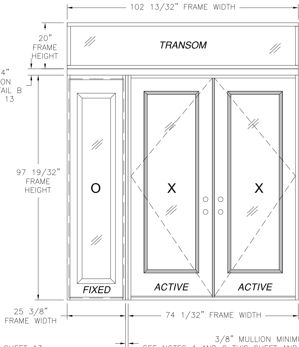
DOUBLE DOOR W/ STD SIDELITE AND TRANSOM EXTERIOR VIEW OXX SHOWN XXO ALSO APPROVED
