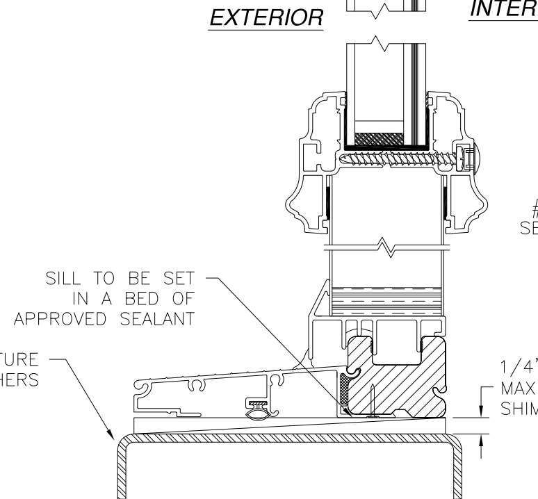
VERTICAL CROSS SECTION DOOR INSTALLATION - METAL STRUCTURE
