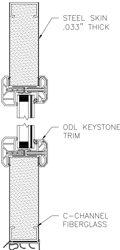
PANEL OPTION 18
