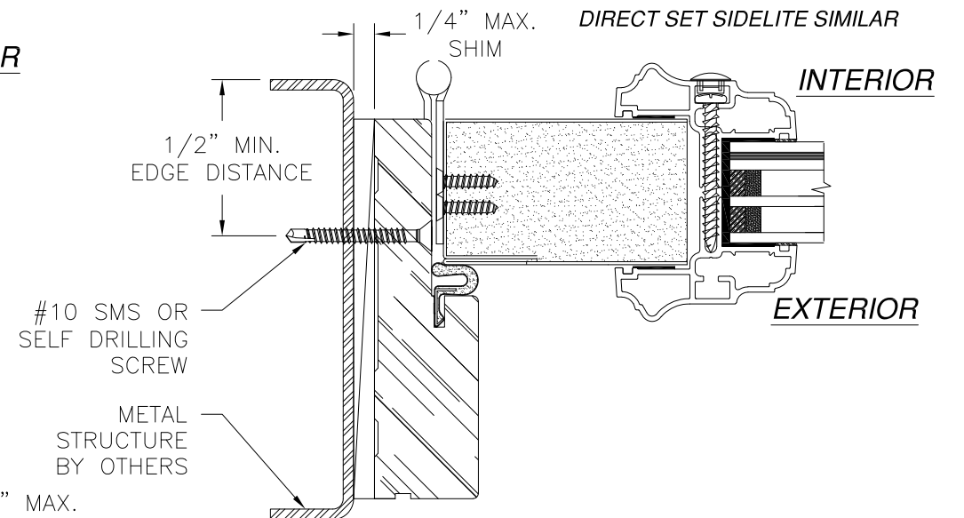
HORIZONTAL CROSS SECTION DOOR INSTALLATION METAL STRUCTURE
