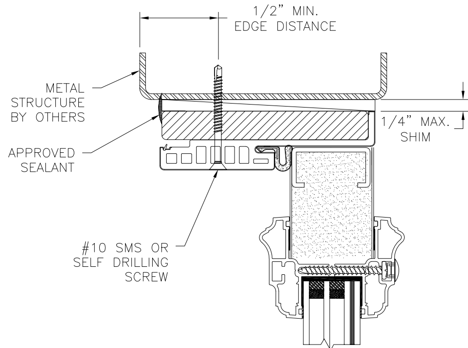
VERTICAL CROSS SECTION STANDARD SIDELITE SHOWN DIRECT SET SIDELITE SIMILAR
