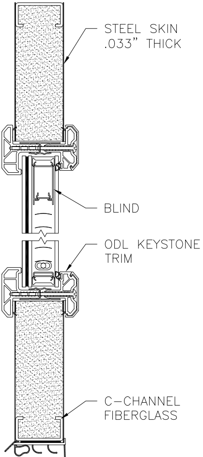
PANEL OPTION 16
