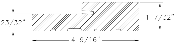
FRAMESAVER COMPOSITE
