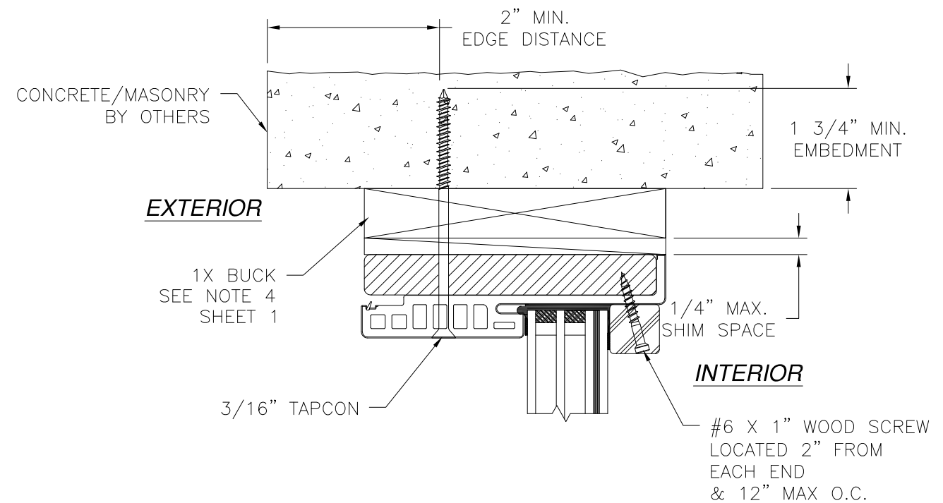
VERTICAL CROSS SECTION TRANSOM INSTALLATION MASONRY/CONCRETE TRANSOM HEAD SHOWN TRANSOM JAMB SIMILAR
