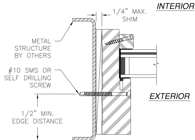
HORIZONTAL CROSS SECTION TRANSOM INSTALLATION METAL STRUCTURE
