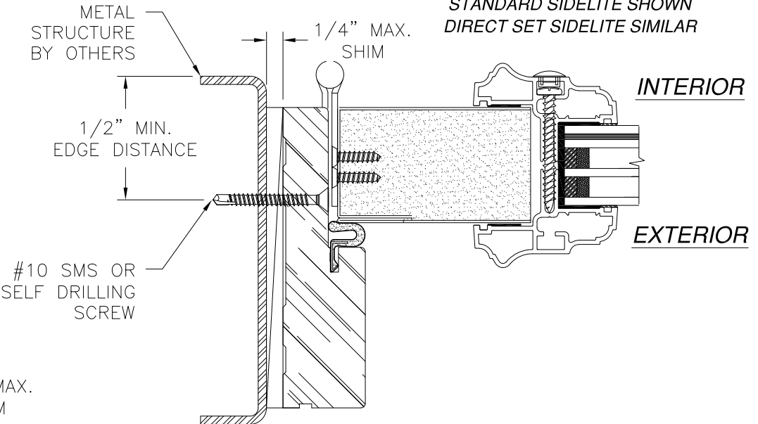
HORIZONTAL CROSS SECTION DOOR INSTALLATION METAL STRUCTURE
