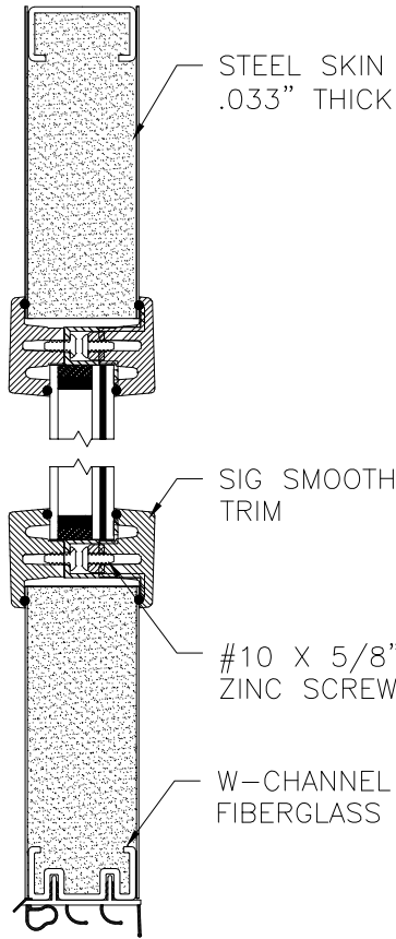
PANEL OPTION 3
