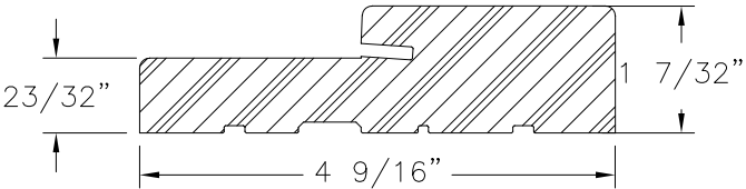
FRAMESAVER COMPOSITE
