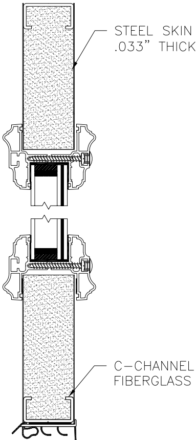
PANEL OPTION 2
