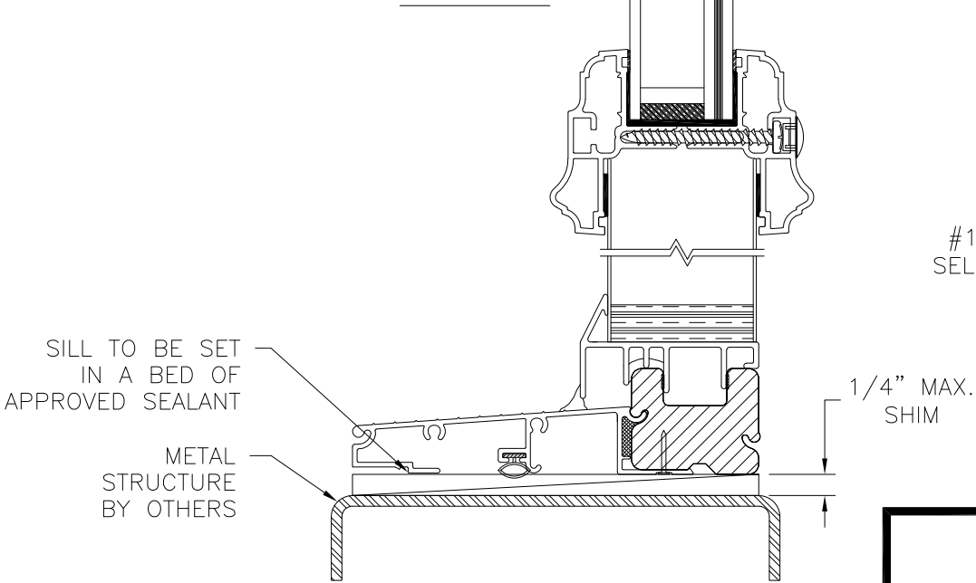
VERTICAL CROSS SECTION SIDELITE INSTALLATION METAL STRUCTURE STANDARD SIDELITE SHOWN DIRECT SET SIDELITE SIMILAR
