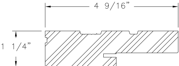
COMPOSITE FRAME PROFILE
