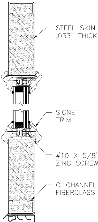
PANEL OPTION 6
