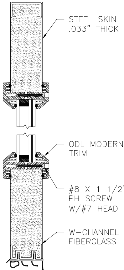
PANEL OPTION 7
