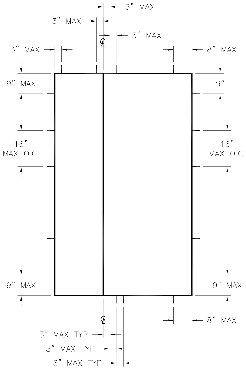
SINGLE W/SIDELITE
