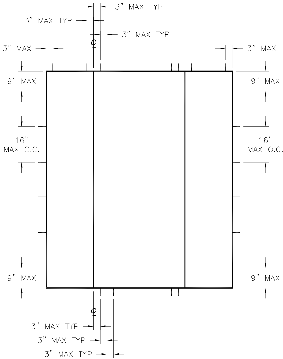
SINGLE W/SIDELITES
