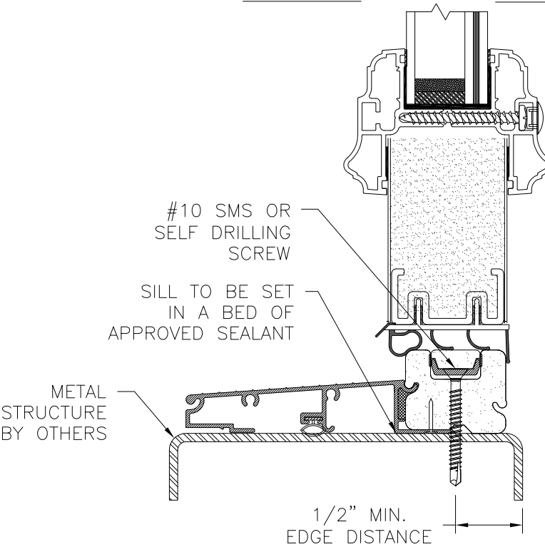
VERTICAL CROSS SECTION DOOR INSTALLATION METAL STRUCTURE
