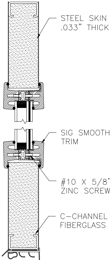
PANEL OPTION 4
