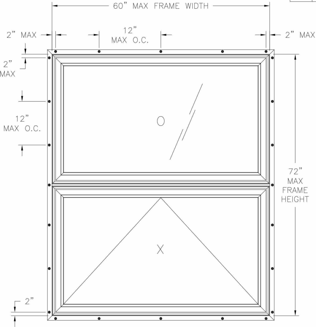
SIGN/CAMB IMP AWNING/FIXED STACKED ASSEMBLY EXTERIOR VIEW FIN INSTALLATION
