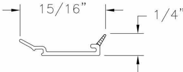
Glazing Bead VINYL PVC .040 THICK
