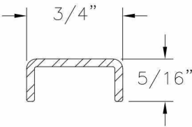
Under Hinge Reinforcement Aluminum 6105 T5, Anodized .060 THICK
