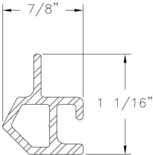
Sash Reinforcement Aluminum 6105 T5, Anodized .078 THICK
