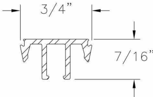
Astragal Reinforcement Aluminum 6105 T5 .060 THICK
