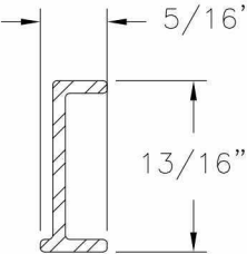
Sash Reinforcement Aluminum 6105 T5, Anodized .060 THICK
