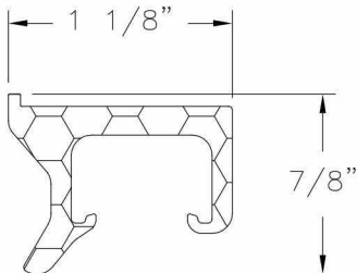
Snubber - Frame Aluminum 6105 T5, Anodized .100 THICK
