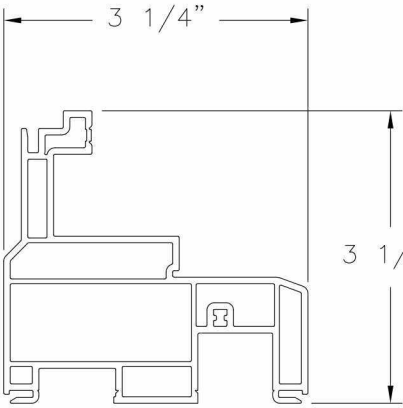
Frame VINYL PVC .070 THICK
