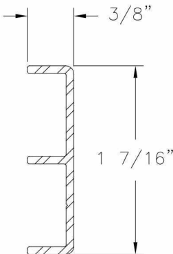
Under Operator Reinforcement Aluminum 6105 T5 .060 THICK
