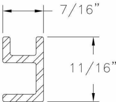
Spacer VINYL PVC .080 THICK
