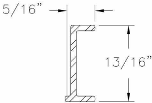
Sash Reinforcement Aluminum 6105 T5, Anodized .060 THICK
