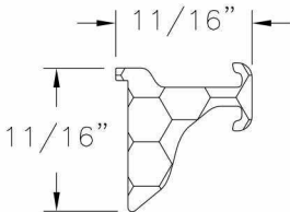
Snubber - Sash Aluminum 6105 T5 .092 THICK
