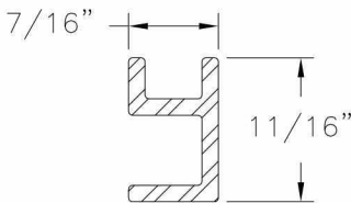
Spacer VINYL PVC .080 THICK
