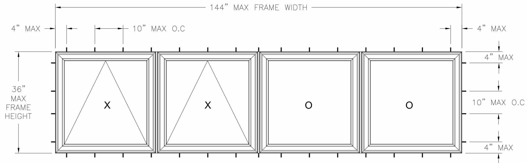
OCEANVIEW IMPACT AW/FIX MULLED ASSEMBLY EXTERIOR VIEW FRAME FLUSH INSTALLATION
