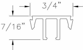
1/2" Mullion VINYL PVC .050 THICK
