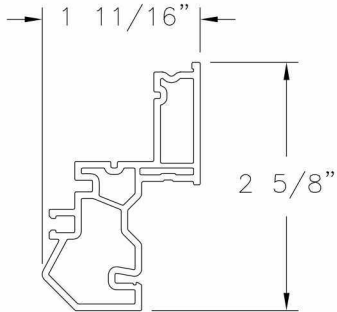
Sash VINYL PVC .070 THICK
