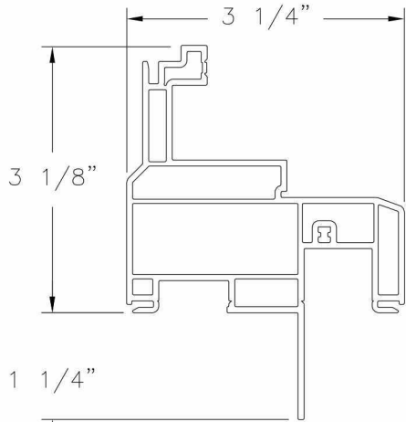
Frame (with Nail Finn) VINYL PVC .070 THICK
