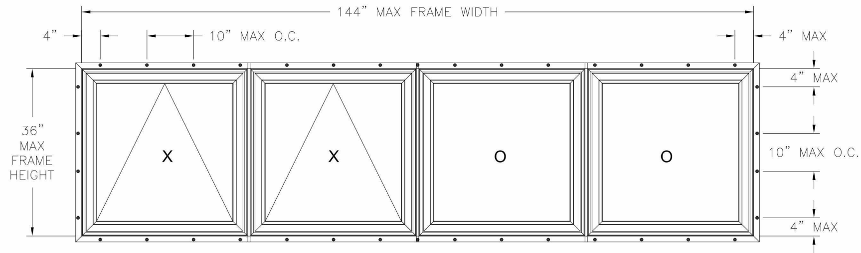
OCEANVIEW IMPACT AW/FIX MULLED ASSEMBLY EXTERIOR VIEW FIN INSTALLATION
