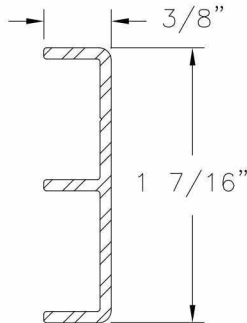
Under Operator Reinforcement Aluminum 6105 T5 .060 THICK
