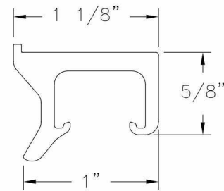
Snubber - Frame Aluminum 6105 T5, Anodized .100 THICK
