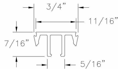
Astragal Reinforcement Aluminum 6105 T5 .060 THICK
