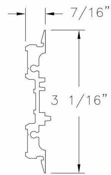
Astragal Reinforcement Aluminum 6105 T5 .060 THICK
