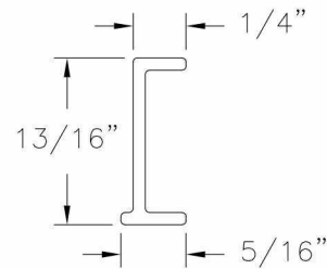
Sash Reinforcement Aluminum 6105 T5, Anodized .060 THICK
