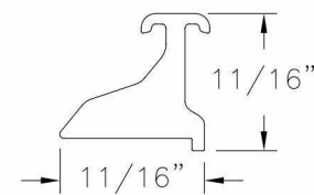
Snubber - Sash Aluminum 6105 T5 .092 THICK
