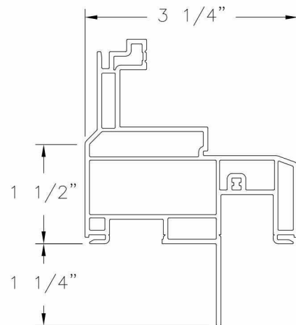
Frame VINYL PVC .070 THICK
