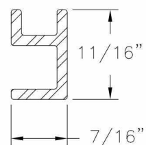
Casement Picture Window Spacer VINYL PVC .080 THICK
