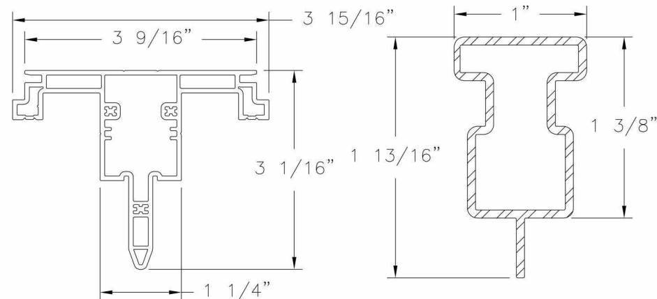
Astragal Frame VINYL PVC .070 THICK
