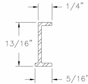
Sash Reinforcement Aluminum 6105 T5, Anodized .060 THICK
