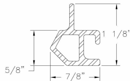
Sash Reinforcement Aluminum 6105 T5, Anodized .078 THICK
