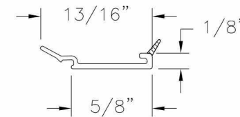
Glazing Bead VINYL PVC .040 THICK
