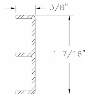
Under Operator Reinforcement Aluminum 6105 T5 .060 THICK
