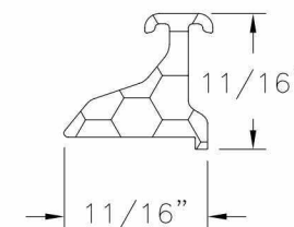
Snubber - Sash Aluminum 6105 T5 .092 THICK
