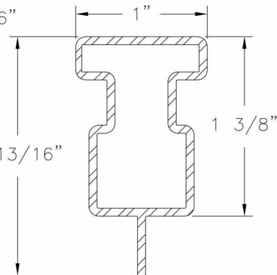
Astragal Reinforcement Aluminum 6105 T5 .060 THICK
