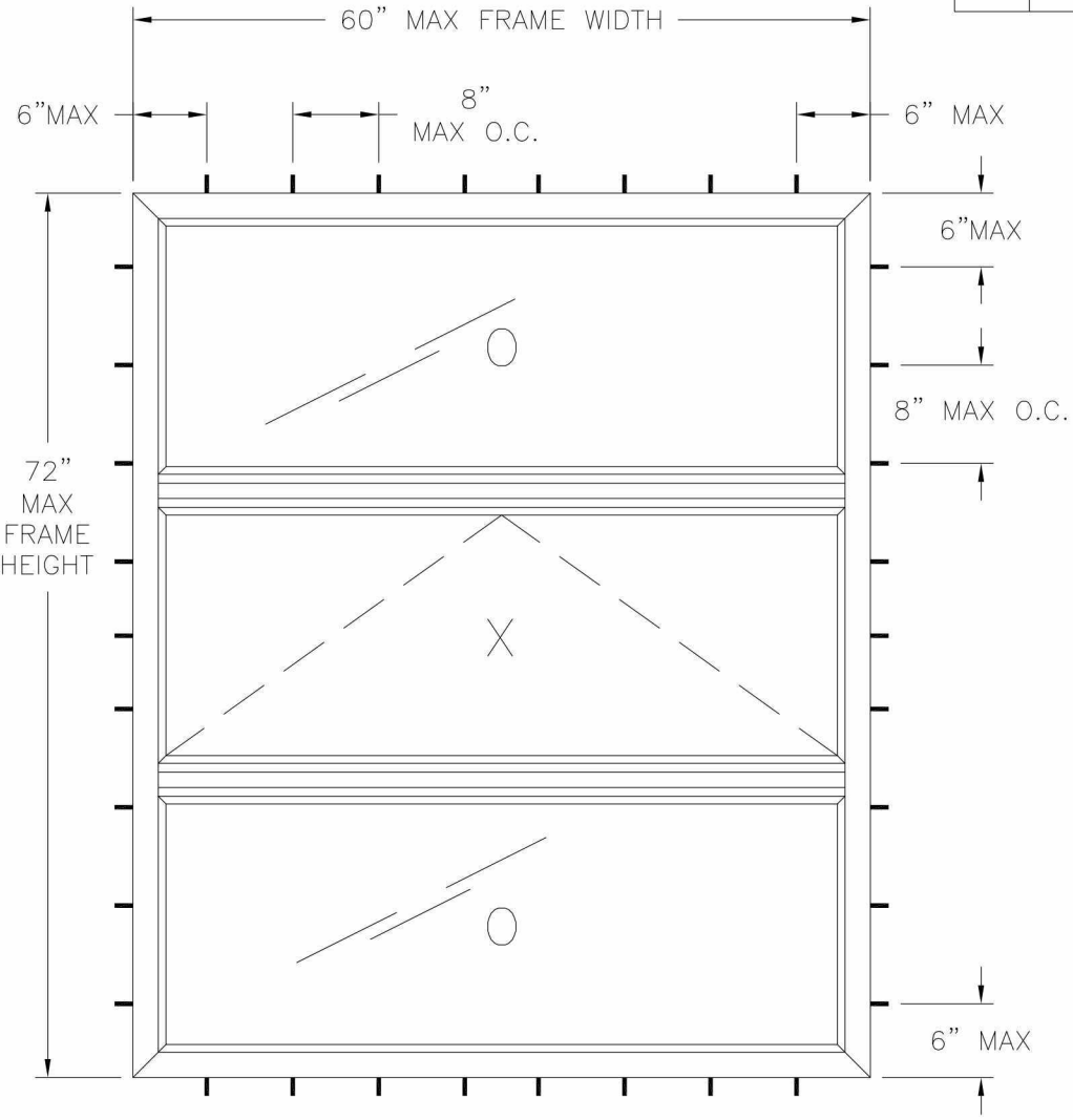
S-SERIES IMPACT AW/ FIX STACKED COMBINATION ASSEMBLY EXTERIOR VIEW FRAME FLUSH INSTALLATION
