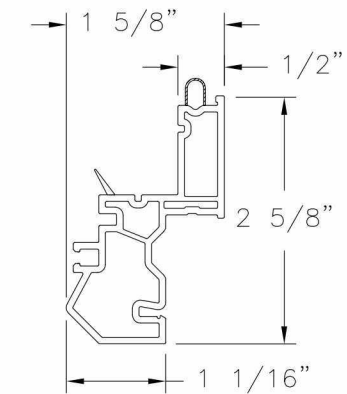
Sash VINYL PVC .070 THICK
