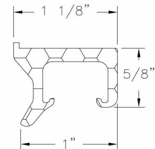
Snubber - Frame Aluminum 6105 T5, Anodized .100 THICK
