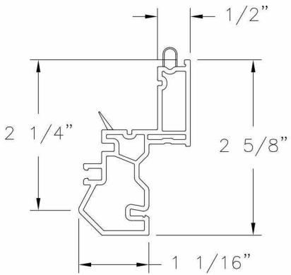
Sash VINYL PVC .070 THICK
