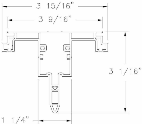
Astragal Frame VINYL PVC .070 THICK
