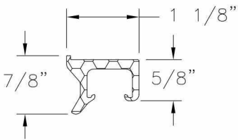
Snubber - Frame Aluminum 6105 T5, Anodized .100 THICK
