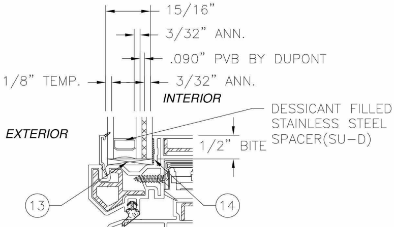
GLAZING DETAIL
