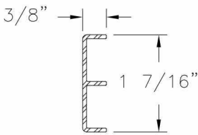
Under Operator Reinforcement Aluminum 6105 T5 .060 THICK
