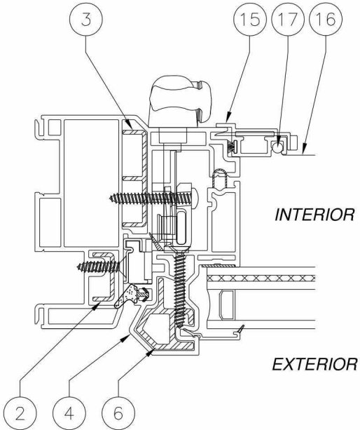
HORIZONTAL SECTION
