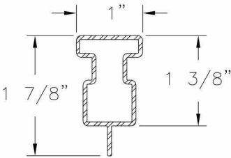
Astragal Reinforcement Aluminum 6105 T5 .060 THICK
