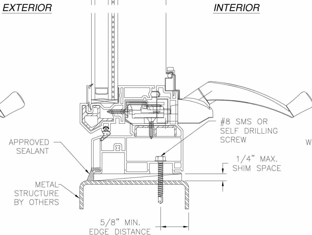
VERTICAL CROSS SECTION METAL STRUCTURE INSTALLATION
