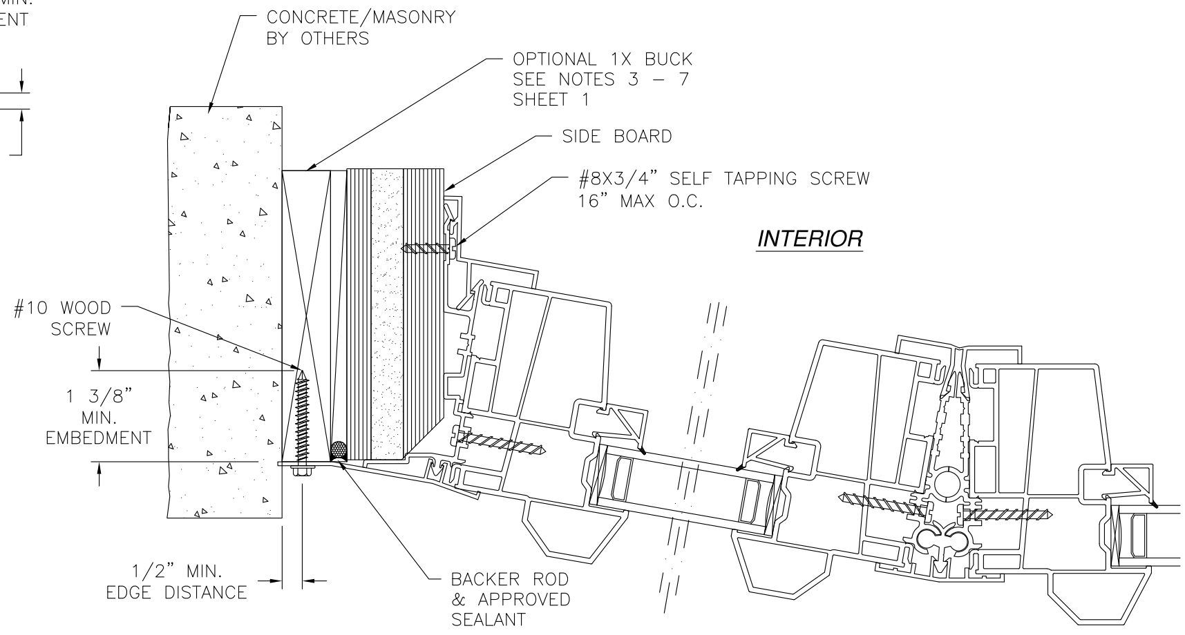
JAMB INSTALLATION DETAIL CONCRETE/MASONRY INSTALLATION
