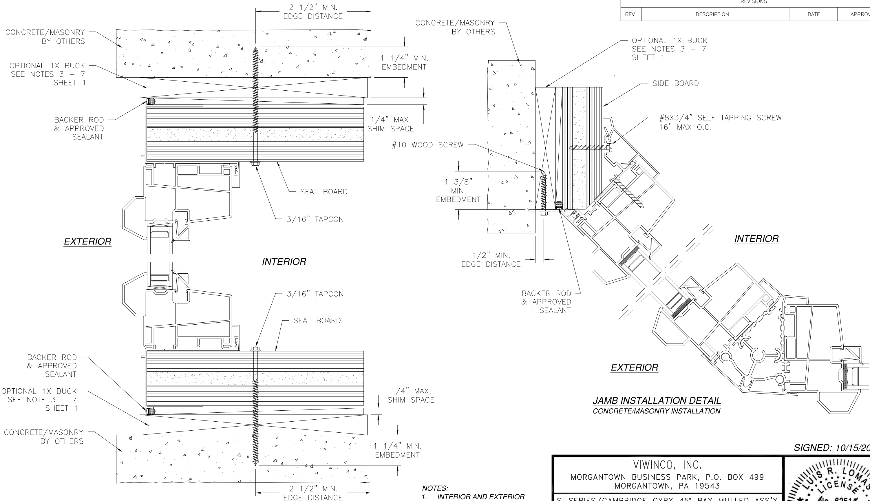
VERTICAL CROSS SECTION CONCRETE/MASONRY INSTALLATION
