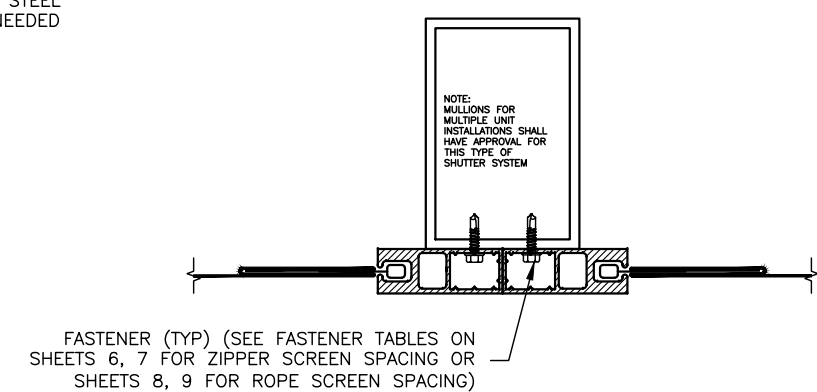
C MULLION MOUNT - SECTION ROLL-UP SCREEN AT MULLIONS - SCALE: N.T.S.
