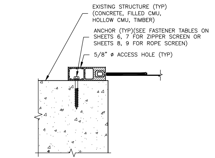
B DIRECT MOUNT - SECTION ROLL-UP SCREEN AT WALL - SCALE: N.T.S.
