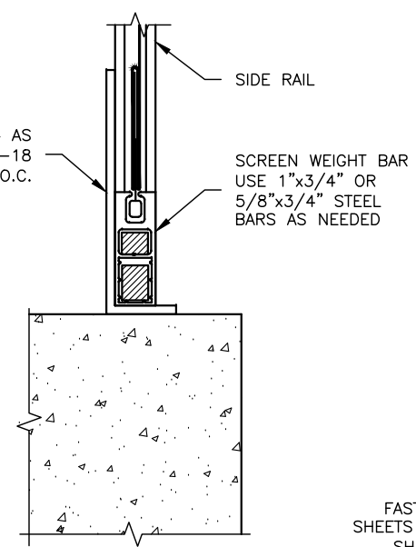
A2 TYPICAL DIRECT MOUNT ROLL-UP SCREEN AT FLOOR - SCALE: N.T.S.
