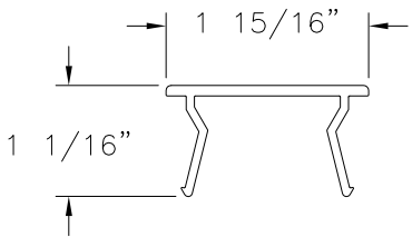
FRAME ADAPTOR PVC EXTRUDED (10003113)
