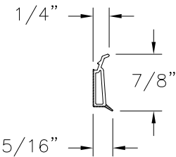
GLAZING BEAD PVC EXTRUDED (10005470)
