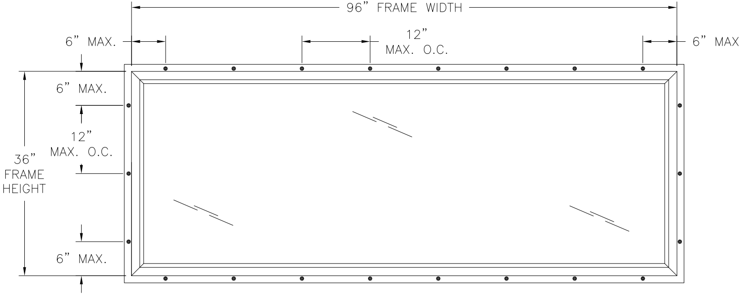
5950 PVC SIDE LITE PICTURE WINDOW EXTERIOR VIEW FIN INSTALLATION
