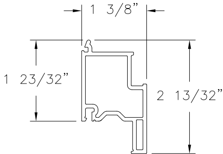
PANEL RISER PVC EXTRUDED (10005862)
