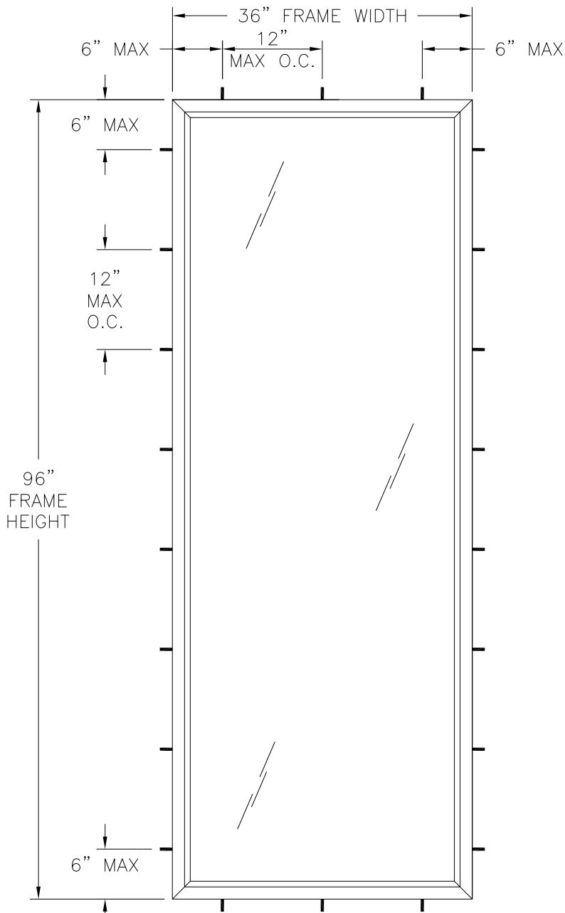
5950 PVC SIDE LITE PICTURE WINDOW EXTERIOR VIEW FRAME INSTALLATION
