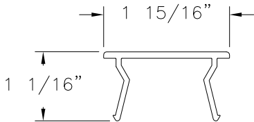
FRAME ADAPTOR PVC EXTRUDED (10003113)
