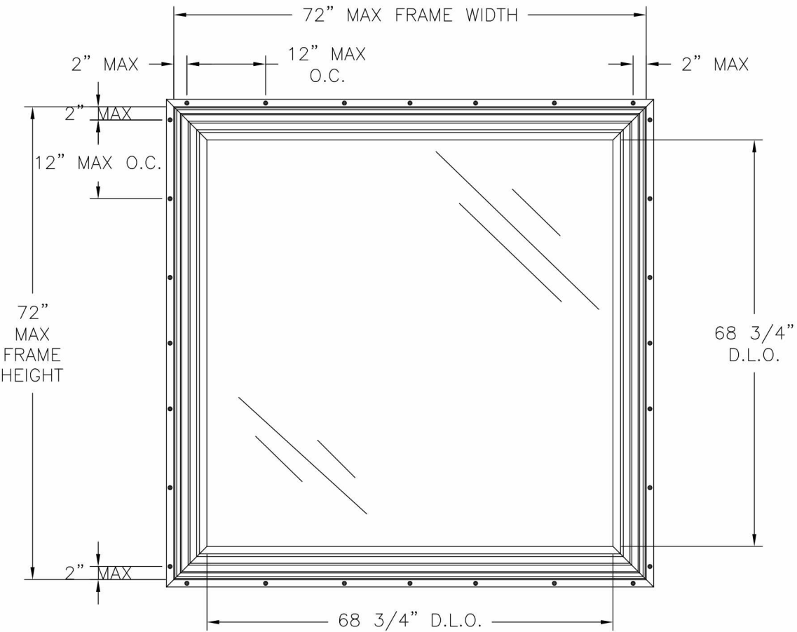
7500 NC FIXED WINDOW FIN INSTALLATION EXTERIOR VIEW
