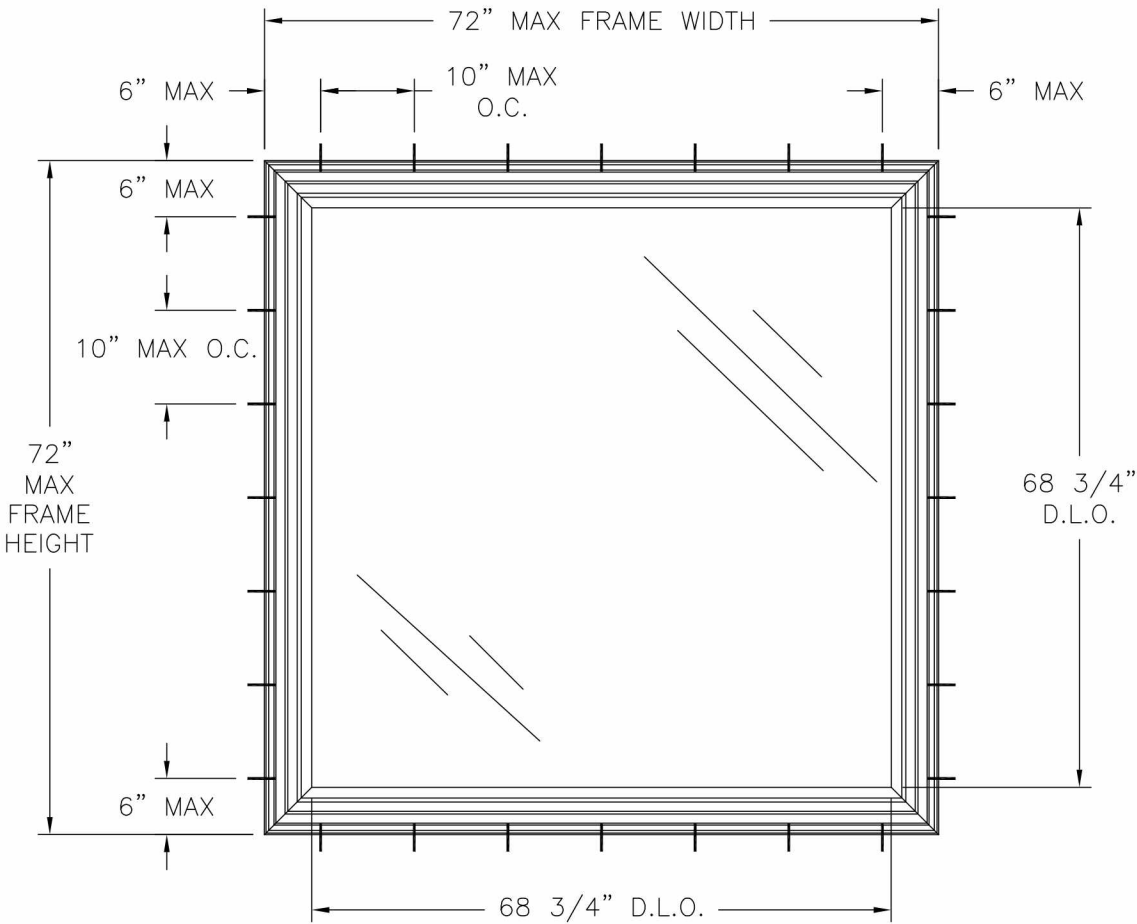
7500 NC FIXED WINDOW FRAME INSTALLATION EXTERIOR VIEW
