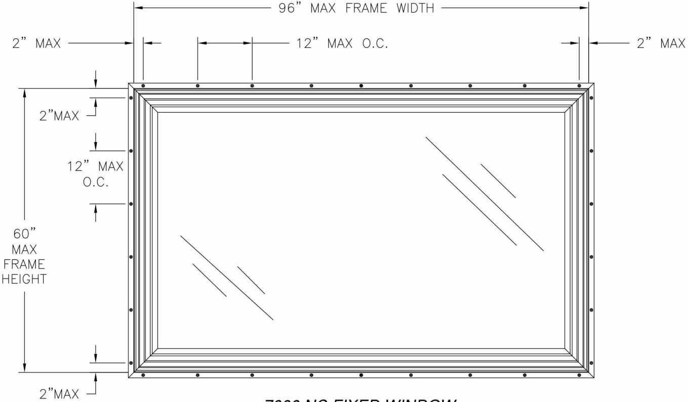
7000 NC FIXED WINDOW FIN INSTALLATION EXTERIOR VIEW
