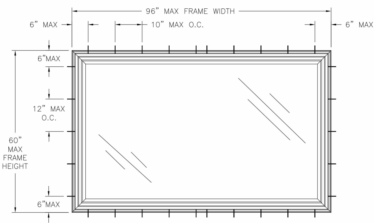
7000 NC FIXED WINDOW FRAME INSTALLATION EXTERIOR VIEW
