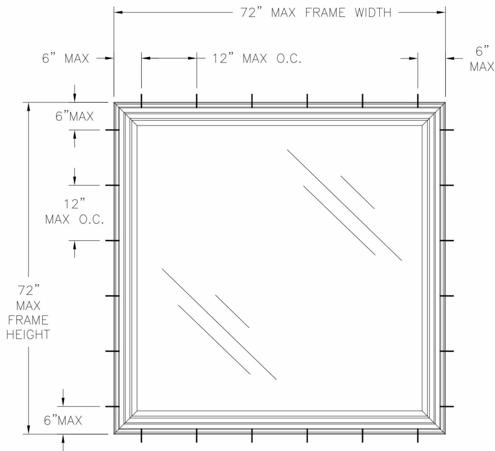
2500/3000 PICTURE WINDOW NON-REINFORCED EXTERIOR VIEW
