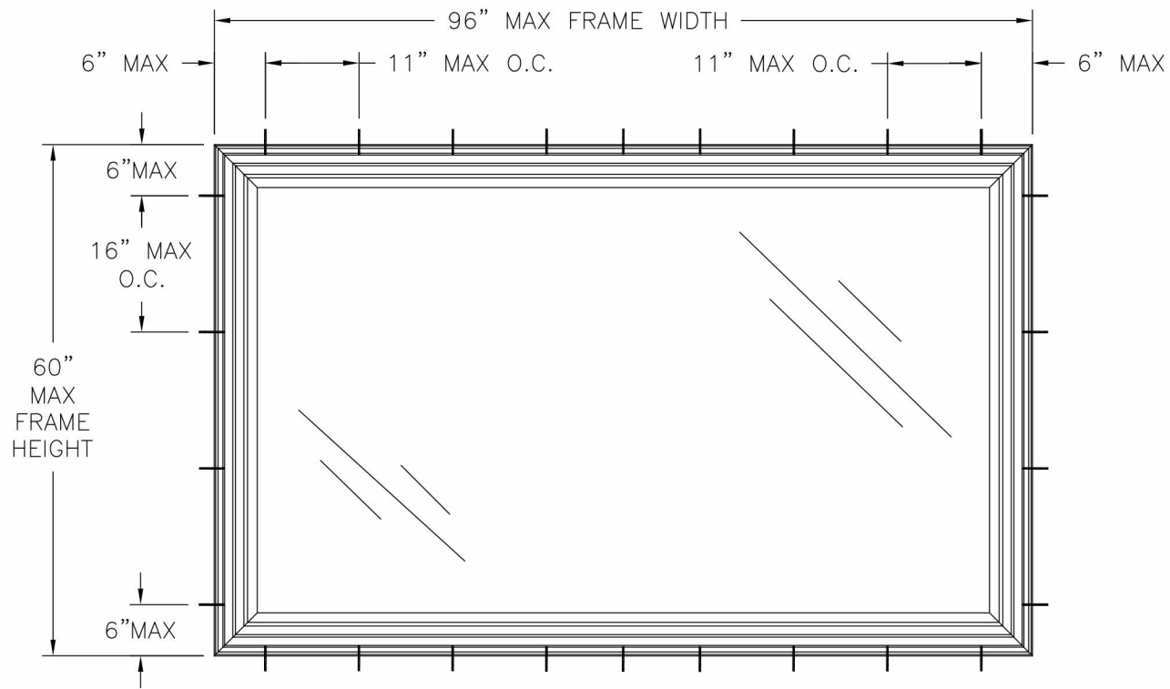
1000 REP FIXED WINDOW EXTERIOR VIEW
