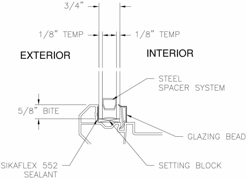
GLAZING DETAIL
