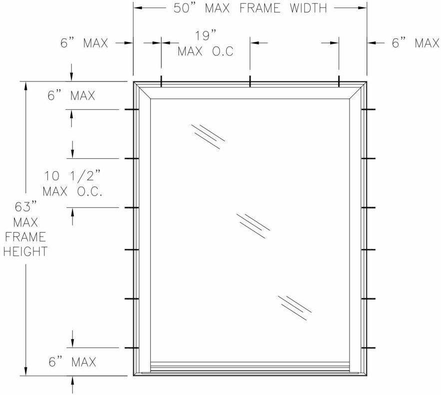
6502 REP FIXED WINDOW EXTERIOR VIEW FRAME INSTALLATION
