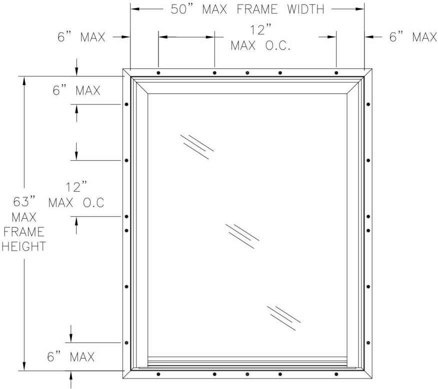
6501 NC FIXED WINDOW EXTERIOR VIEW FIN INSTALLATION
