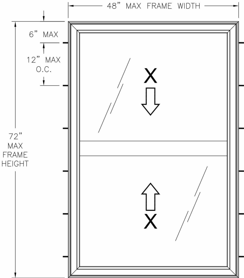
2745 DOUBLE HUNG WINDOW EXTERIOR VIEW FRAME INSTALLATION
