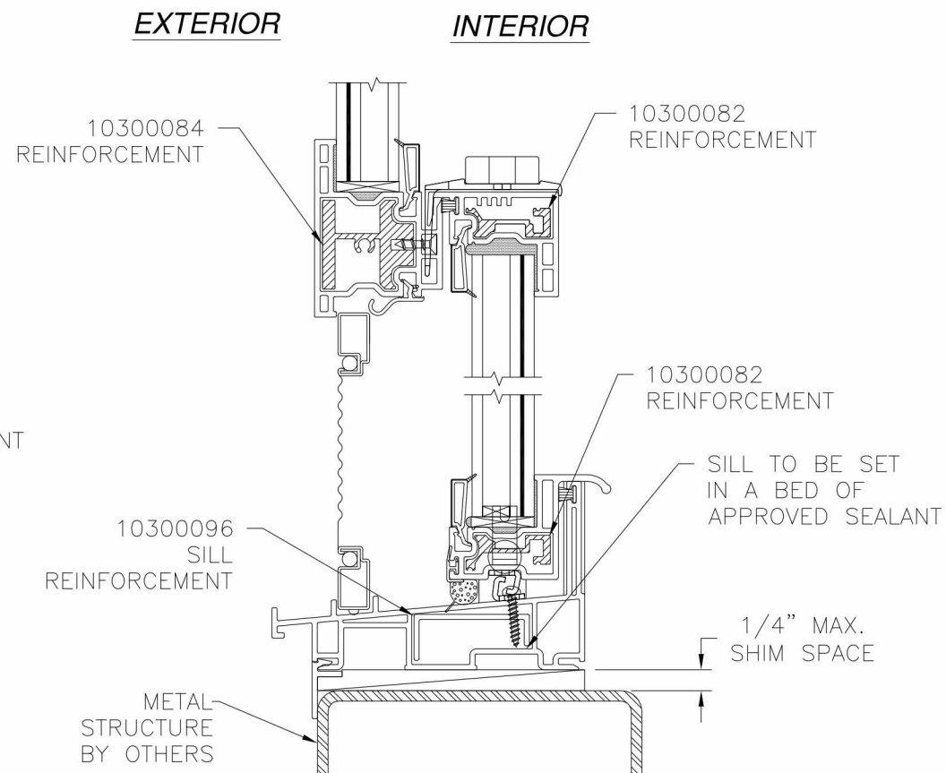
VERTICAL CROSS SECTION METAL STRUCTURE INSTALLATION
