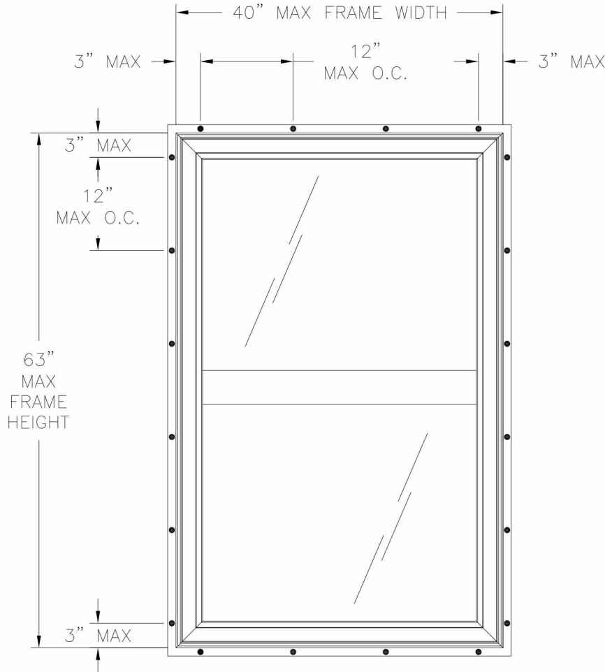
7100 NC SINGLE HUNG WINDOW EXTERIOR VIEW FIN INSTALLATION
