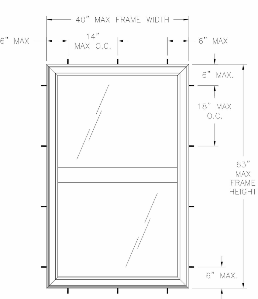
7100 NC SINGLE HUNG WINDOW EXTERIOR VIEW FRAME INSTALLATION
