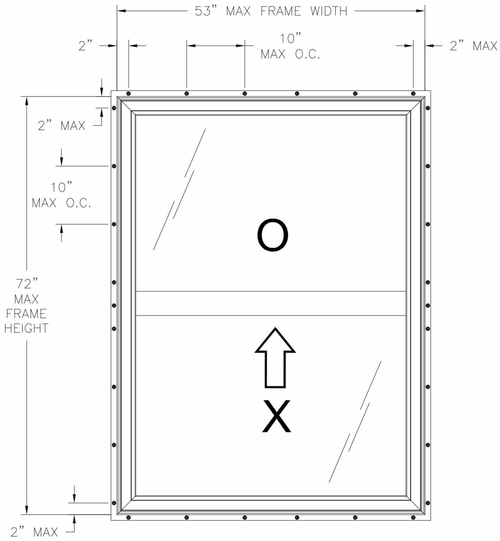
6602 REP SINGLE HUNG WINDOW EXTERIOR VIEW FIN INSTALLATION
