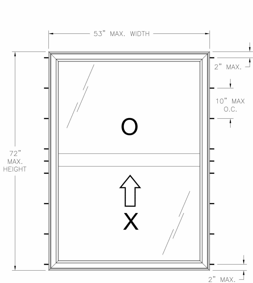
6602 REP SINGLE HUNG WINDOW EXTERIOR VIEW FRAME INSTALLATION
