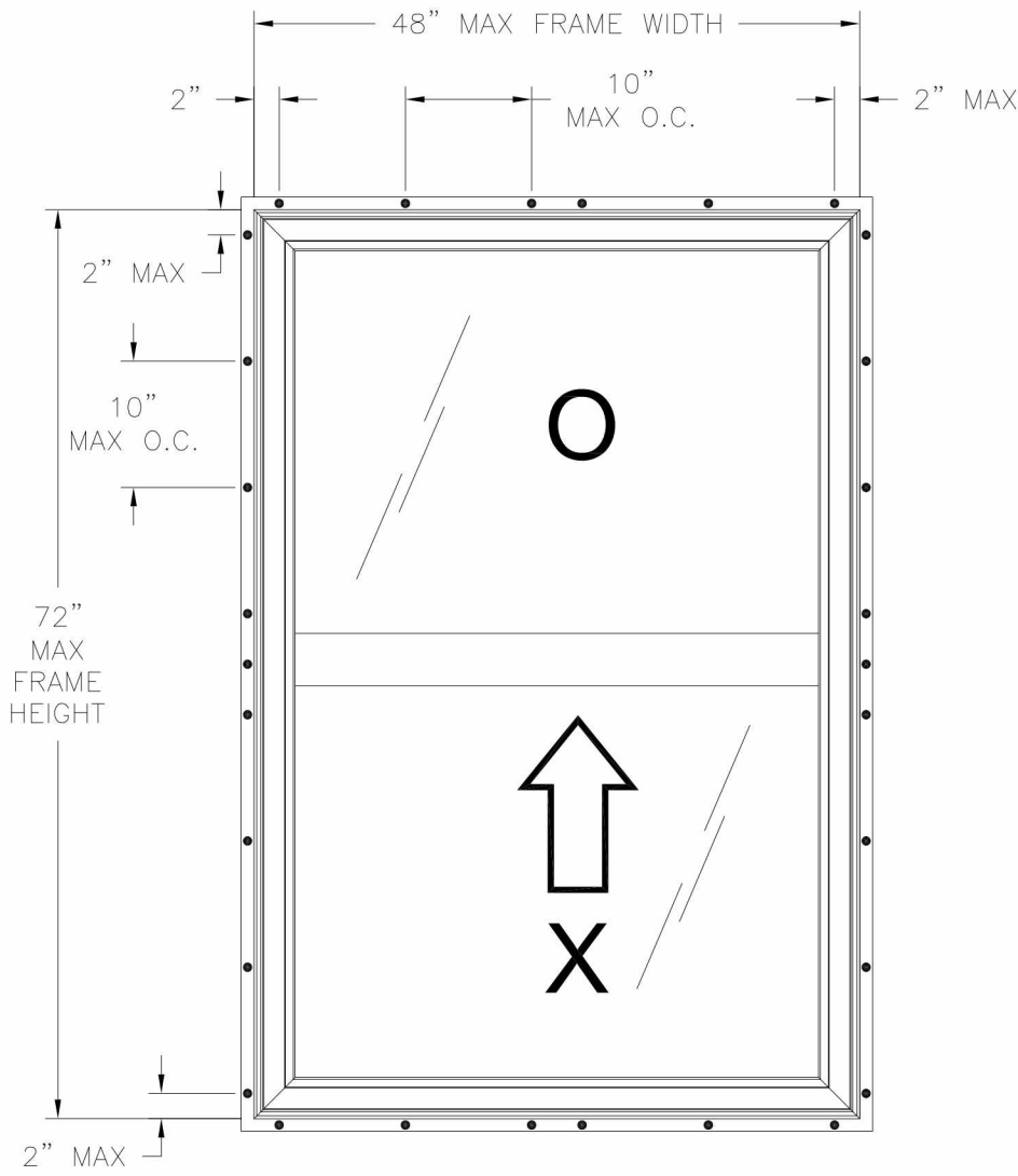
6101NC IMPACT SINGLE HUNG WINDOW EXTERIOR VIEW FIN INSTALLATION
