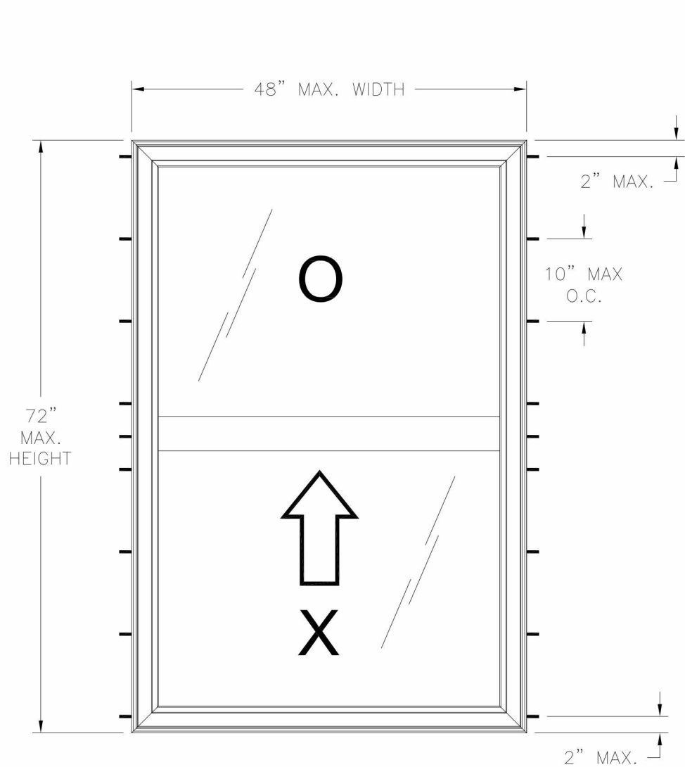
6101NC IMPACT SINGLE HUNG WINDOW EXTERIOR VIEW FRAME INSTALLATION
