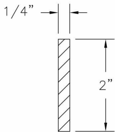
4 MULLION REINFORCEMENT STEEL 1/4" THICK
