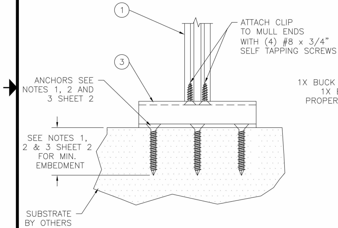
ALTERNATE MULL CLIP 10300093 INSTALLATION DETAILS SILL, SHOWN, HEAD AND JAMBS SIMILAR.
