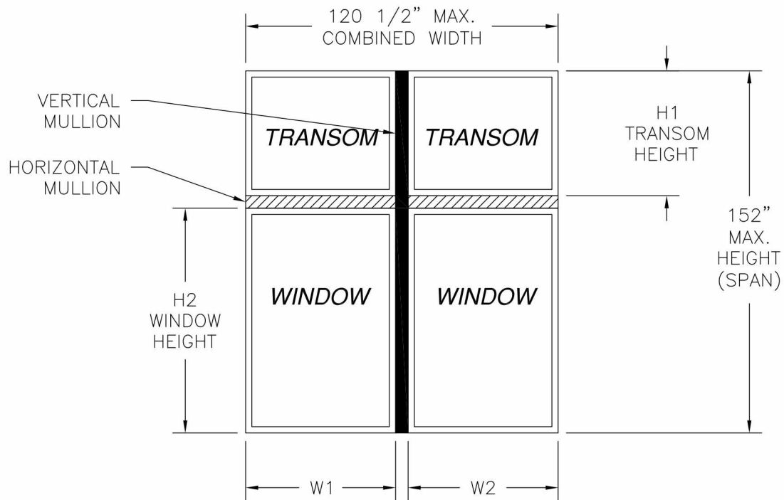
10300085 ALUMINUM X MULLION REINFORCED LMI WIND ZONE 3
