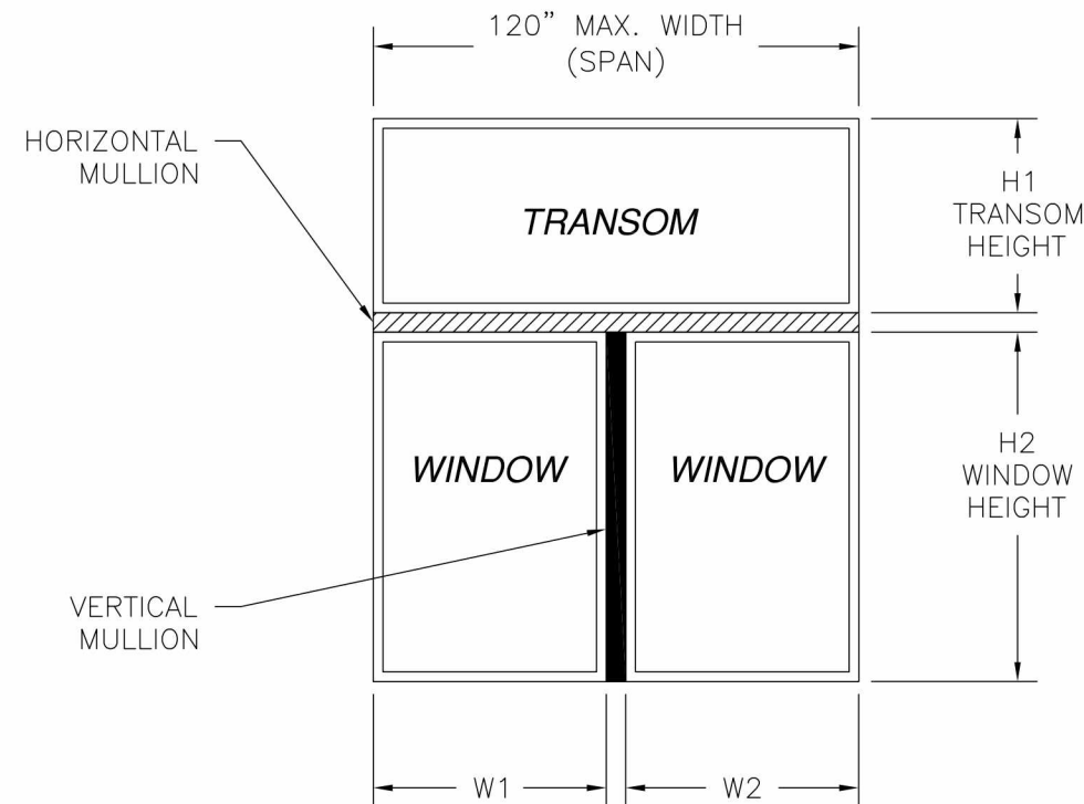
10300085 ALUMINUM T MULLION REINFORCED LMI WIND ZONE 3
