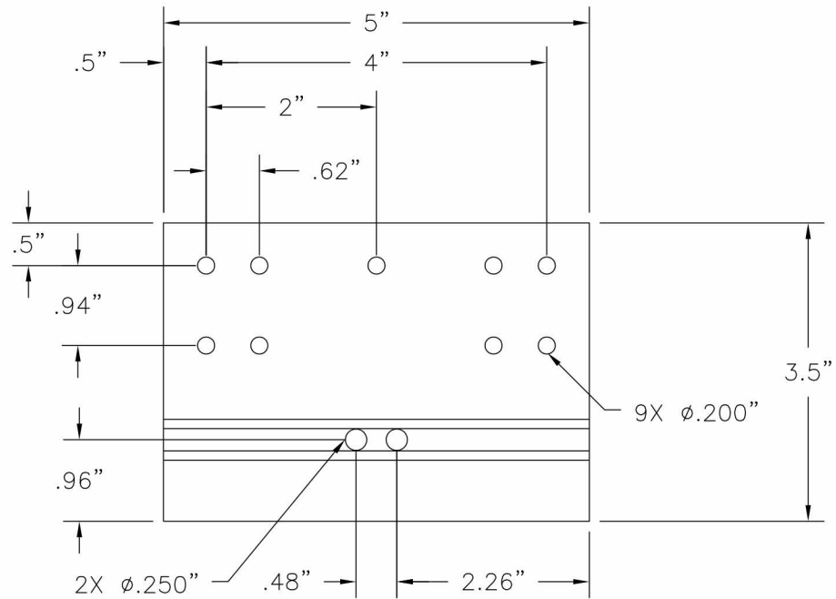
2 STEEL MULLION BRACKET 15GA. GALVANIZED STEEL
