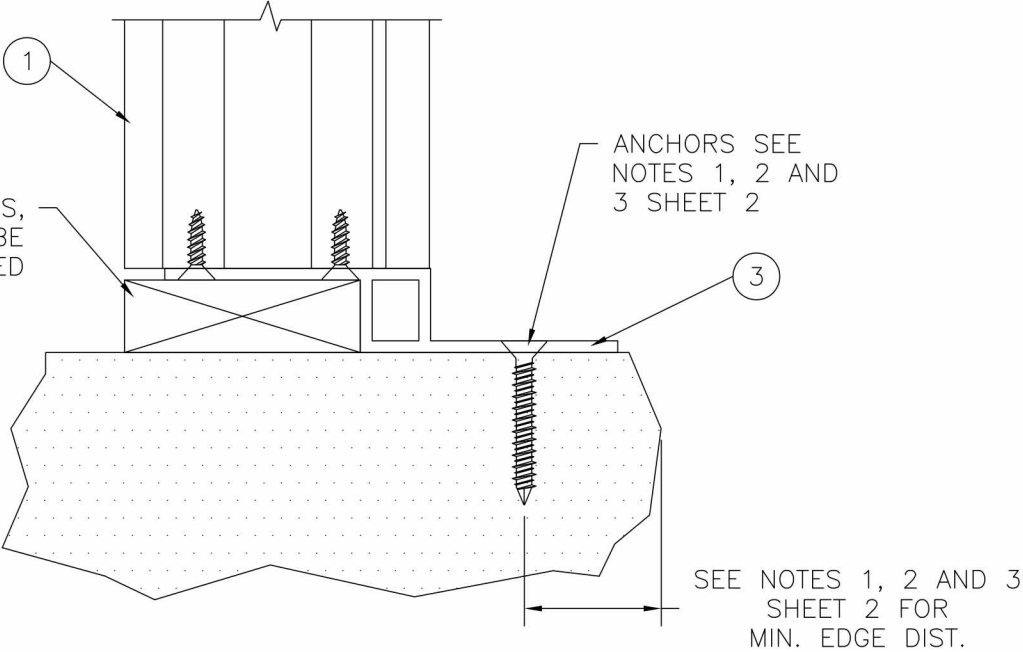
ALTERNATE MULL CLIP 10300093 INSTALLATION DETAILS SILL, SHOWN, HEAD AND JAMBS SIMILAR
