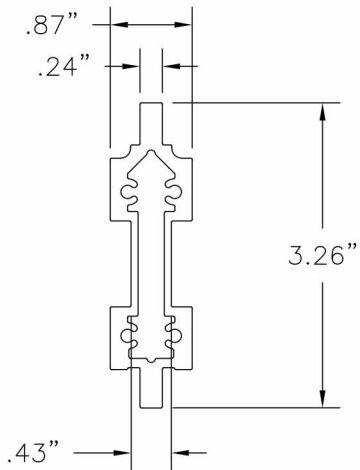
1 10300085 ALUMINUM VERTICAL MULLION ALUMINUM 6005-T5 .075" THICK MINIMUM
